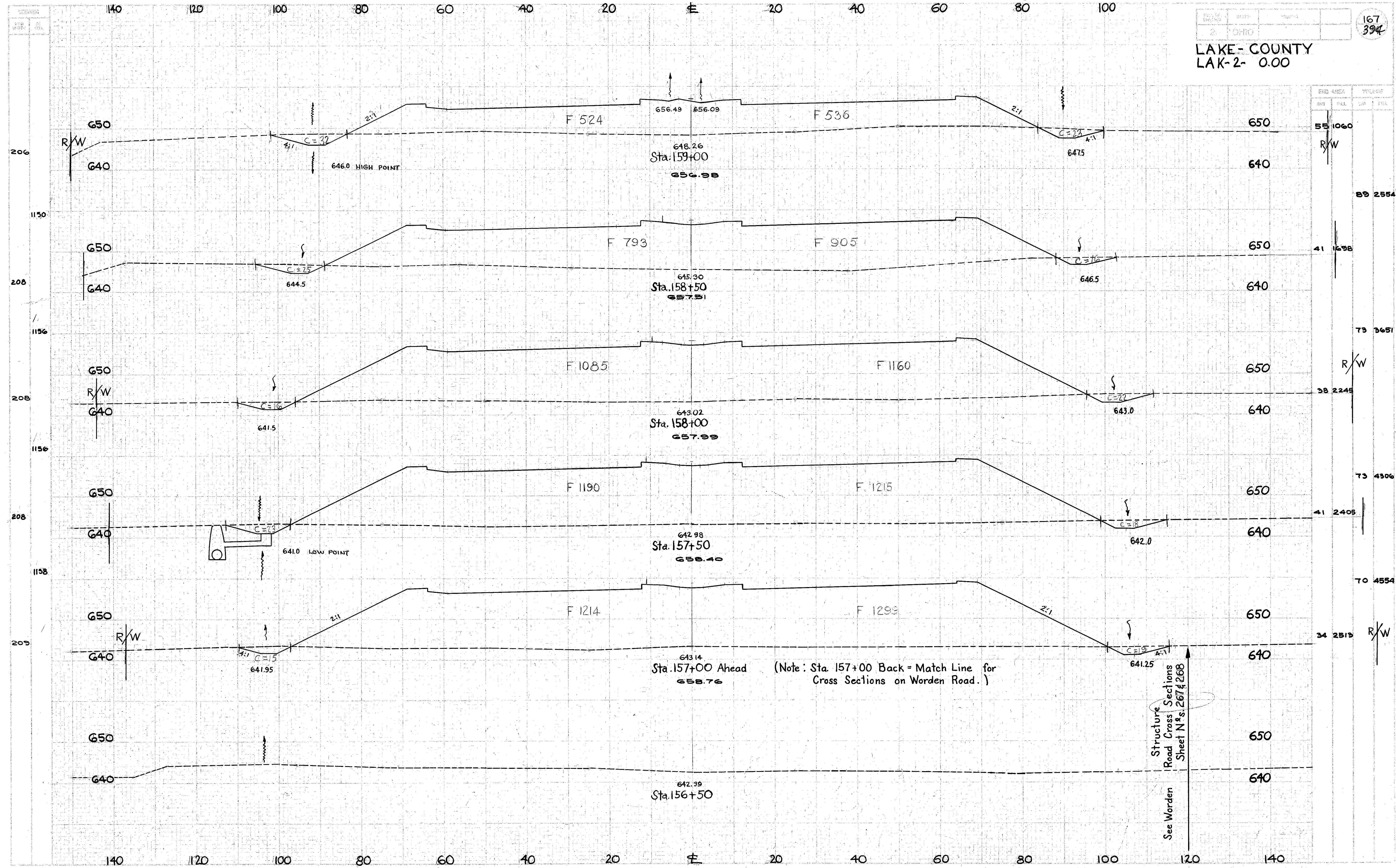
CROSS SECTIONS- STA.156+50 TO STA.159+00
