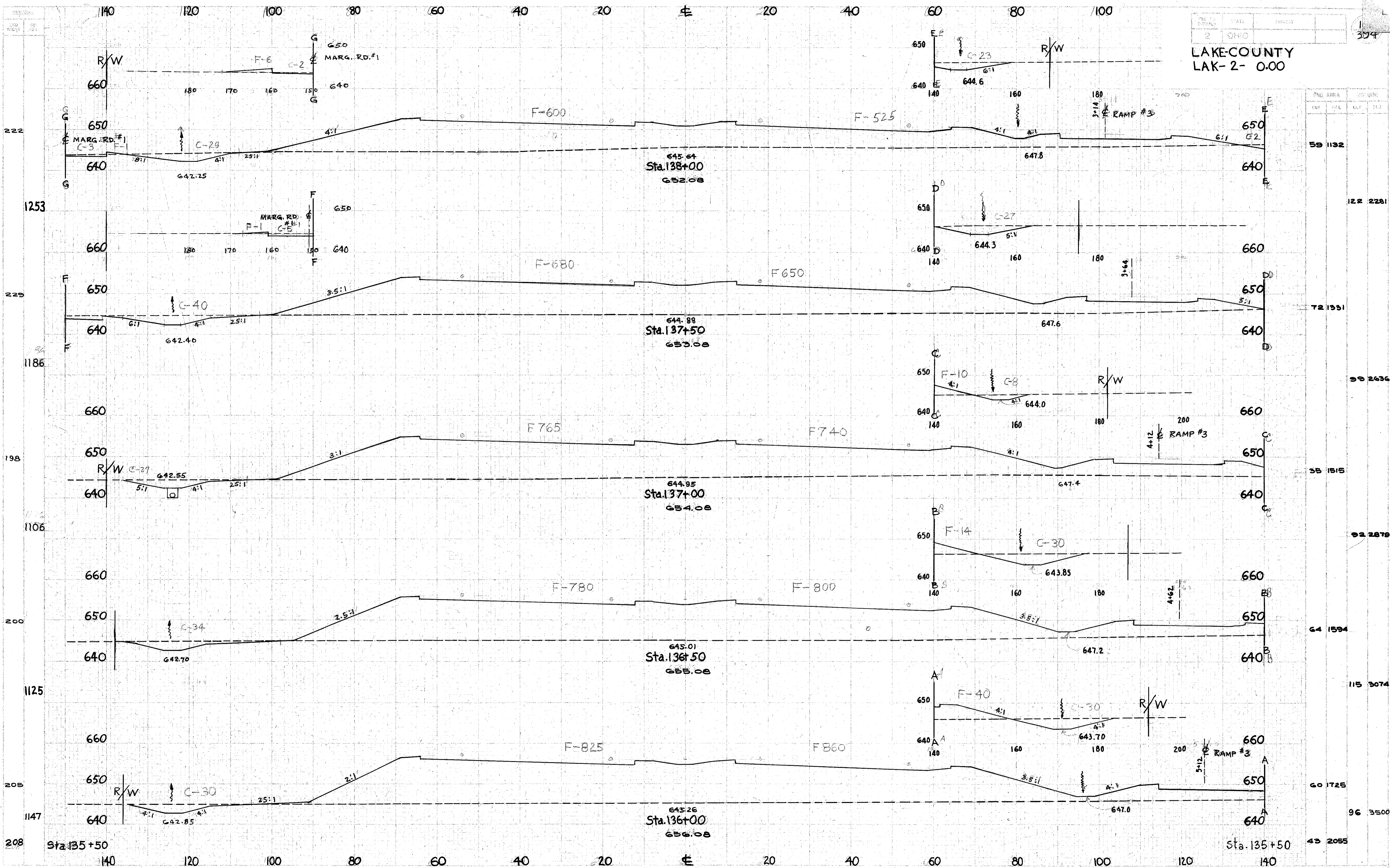
CROSS SECTIONS-STA.136+00 TO STA.138+00
