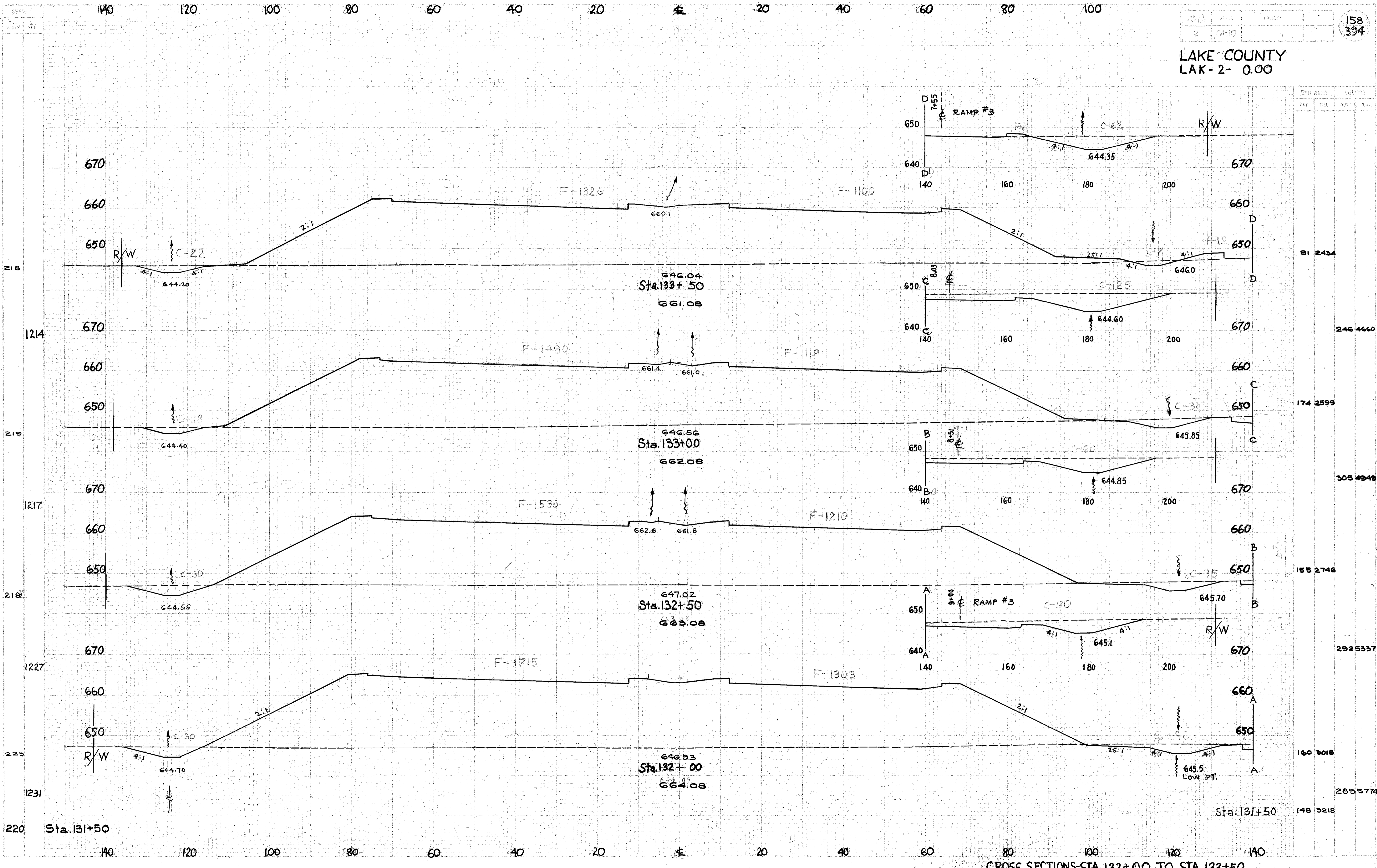
CROSS SECTIONS-STA.132+00 TO STA.133+50
