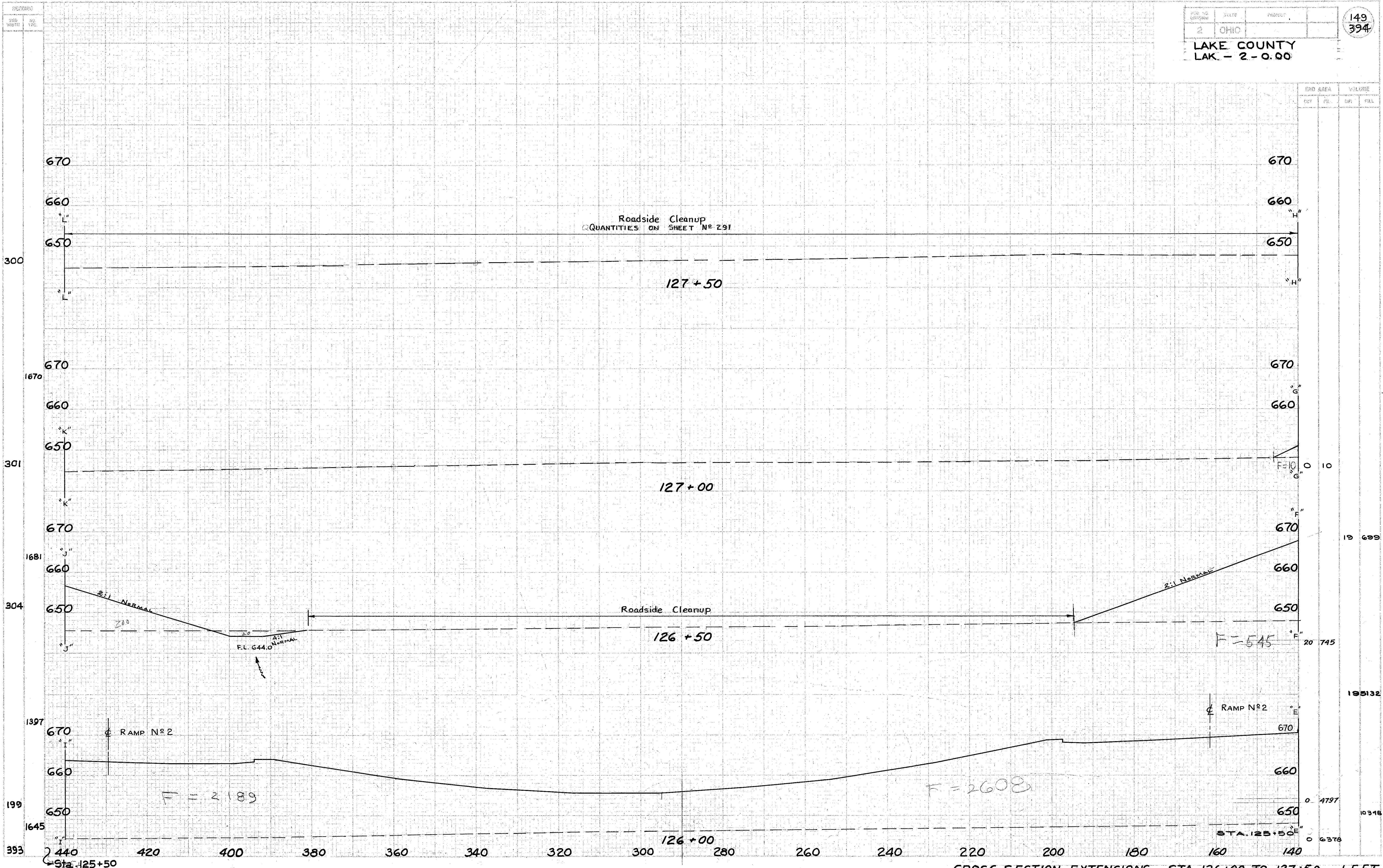
CROSS SECTION EXTENSIONS - STA. 126+00 TO 127+50 - LEFT
