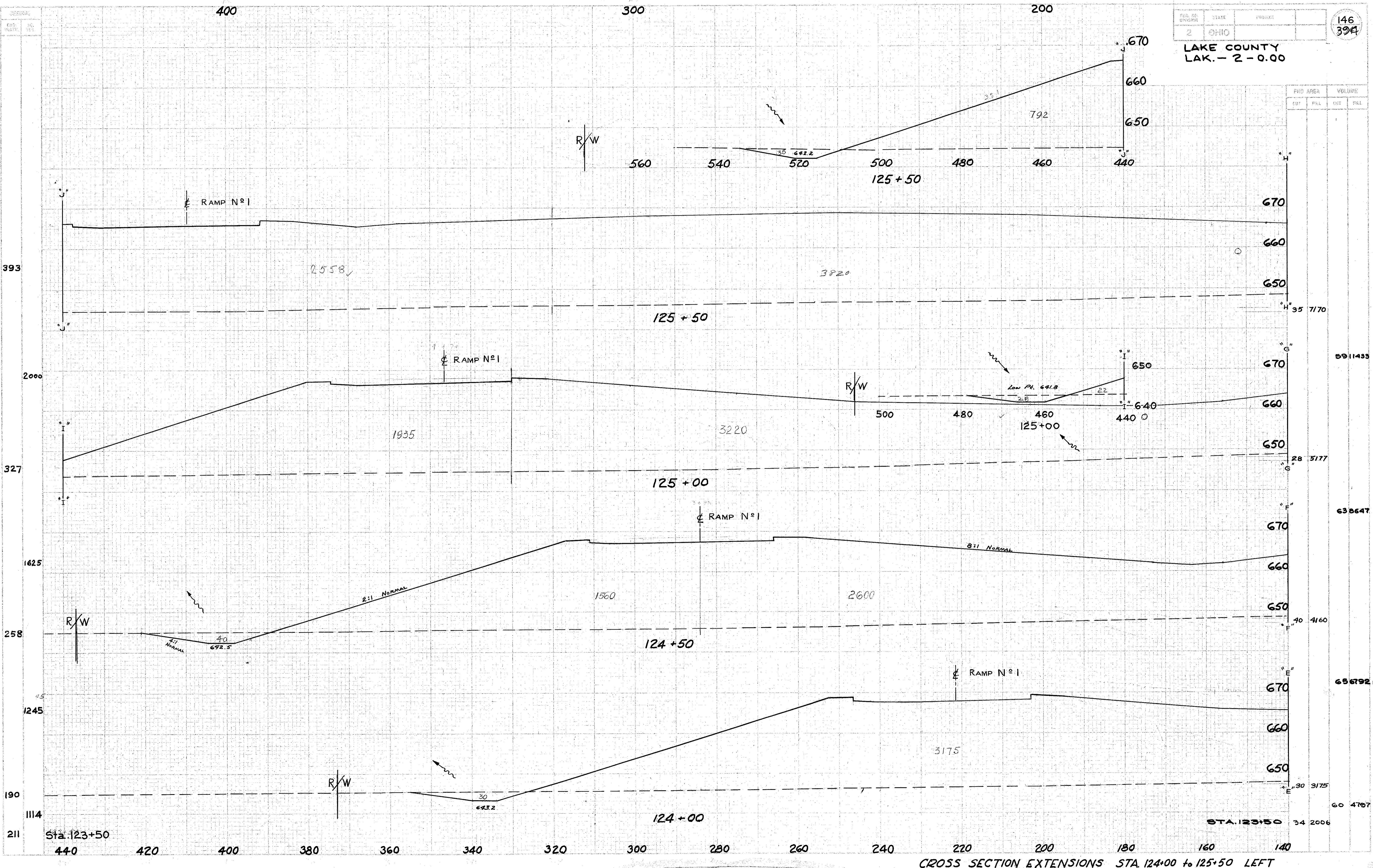
CROSS SECTION EXTENSIONS STA. 124+00 to 125+50 LEFT
