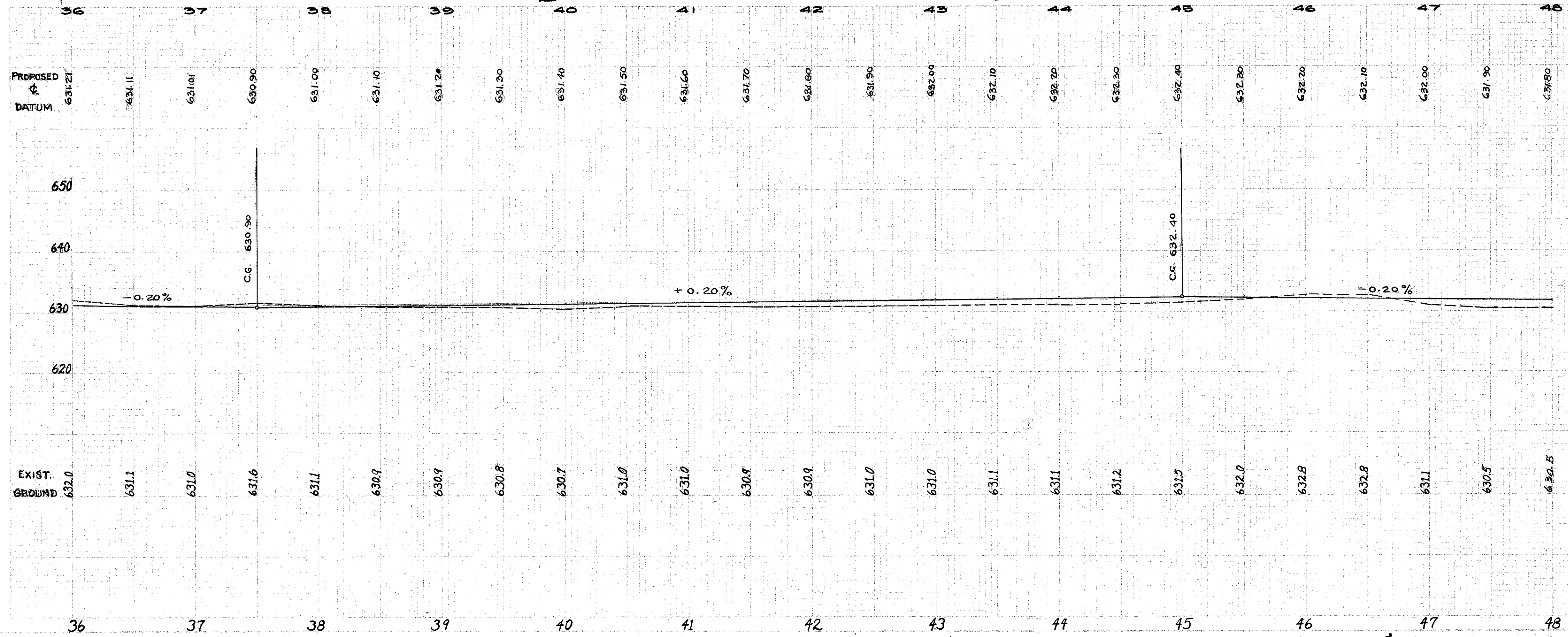
PLAN & PROFILE MARGINAL RD. N o 3 STA. 36+00 TO STA. 48+00
