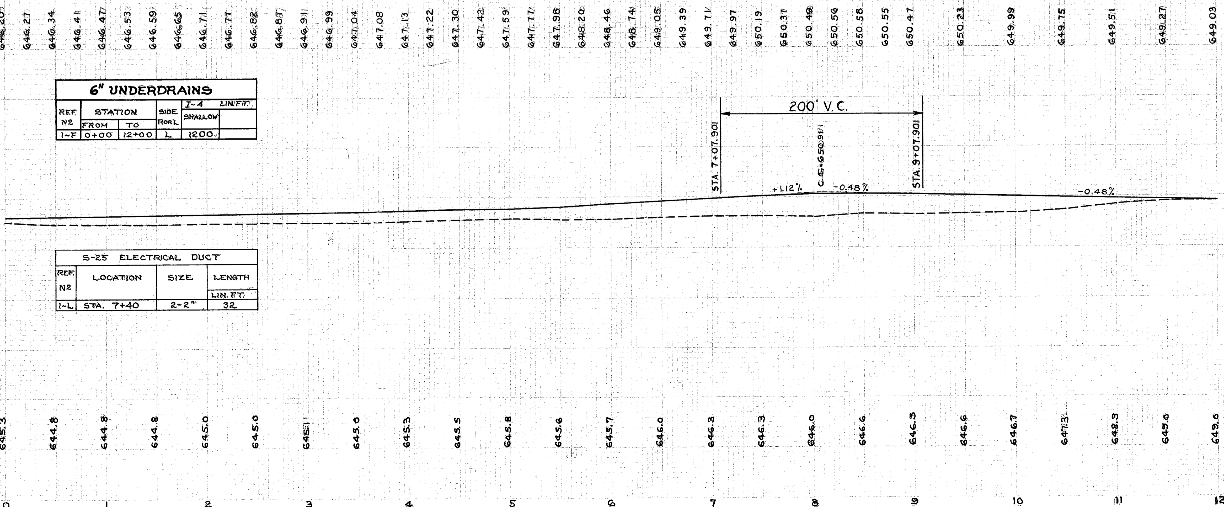
PLAN & PROFILE... RAMP No 7 STA.0+00 TO STA.12+00
