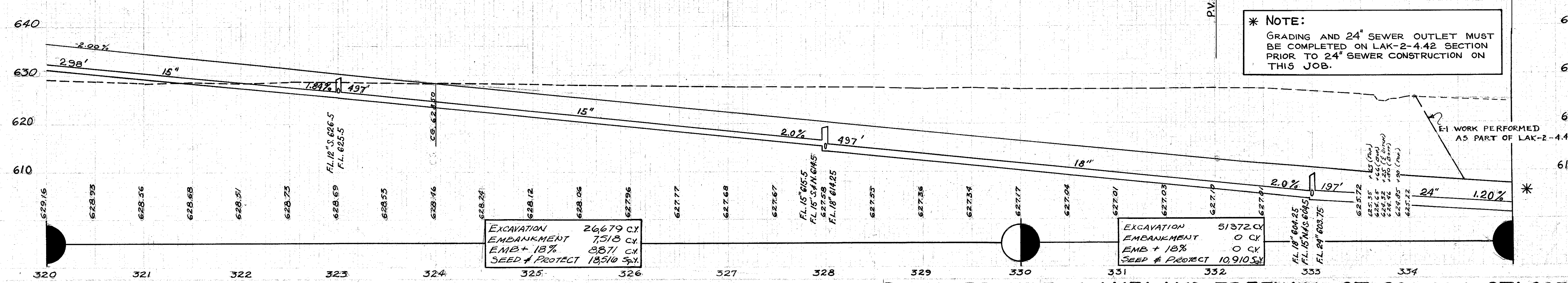
PLAN & PROFILE LAKELAND FREEWAY STA. 320+00 to STA. 335+05.71
