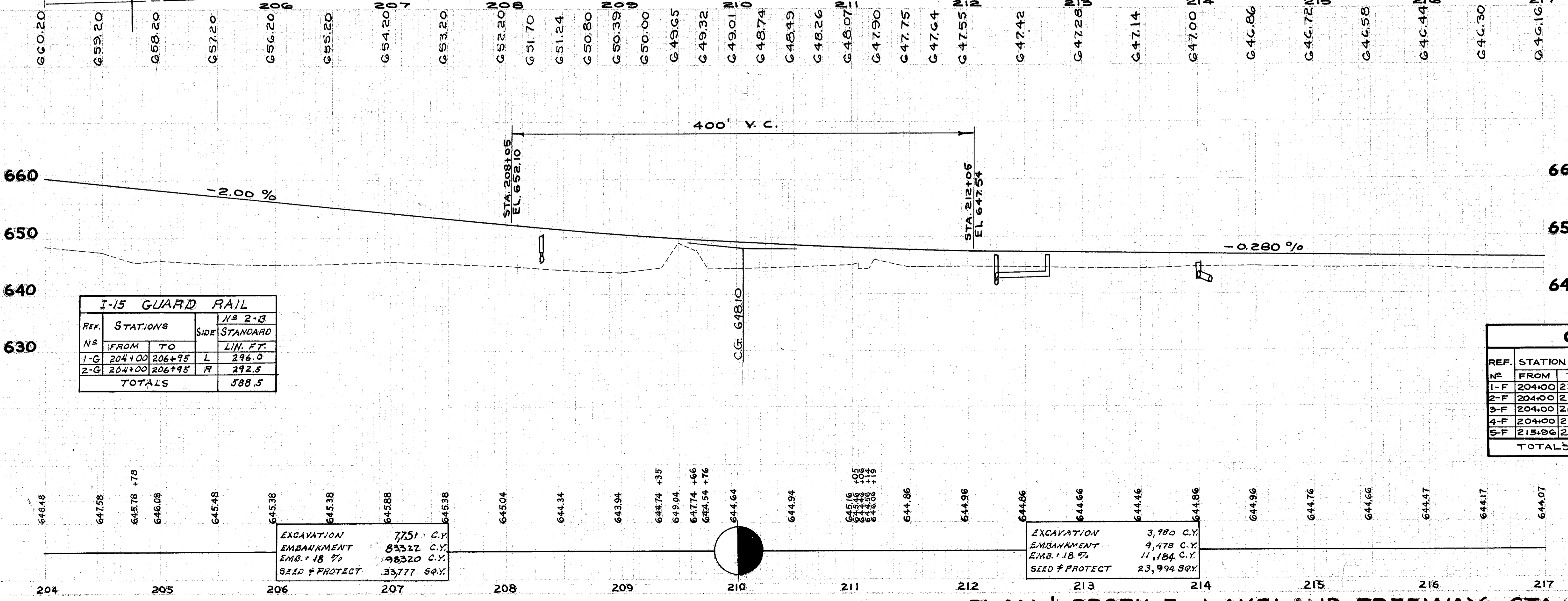
PLAN & PROFILE - LAKELAND FREEWAY - STA. 204+00 TO STA. 217+00
