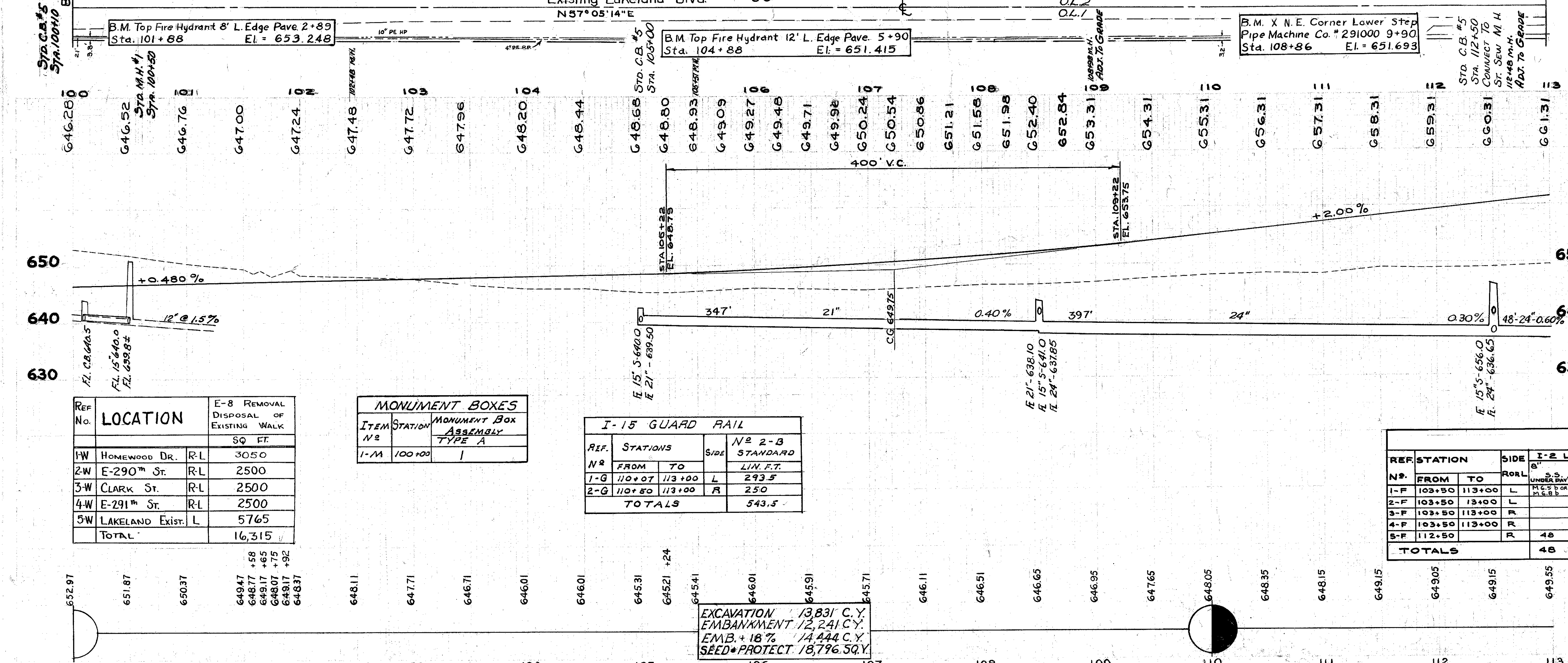
PLAN & PROFILE LAKELAND FREEWAY STA. 100+00 TO STA. 113+00
