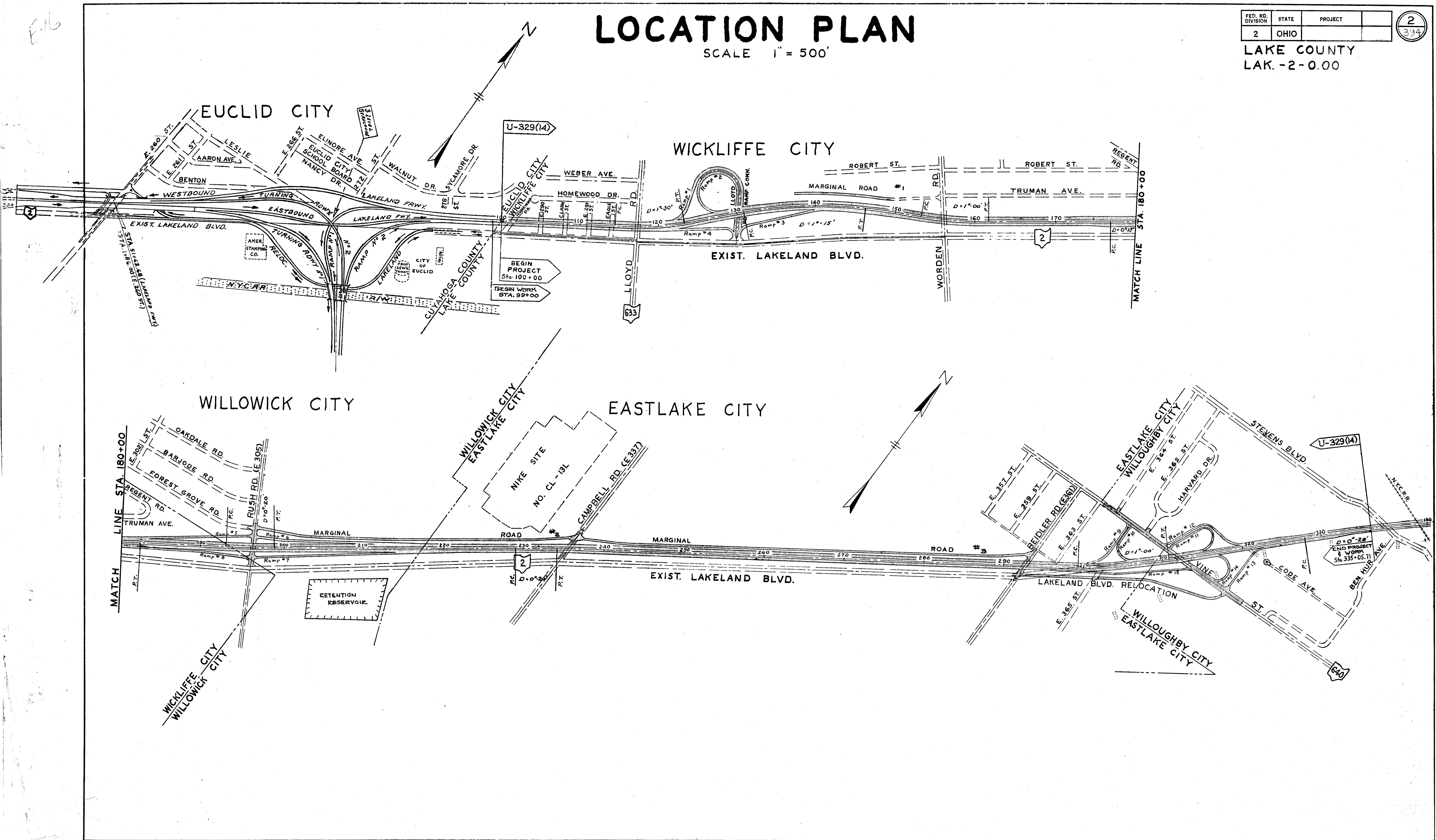
LAKELAND FREEWAY - LOCATION PLAN
