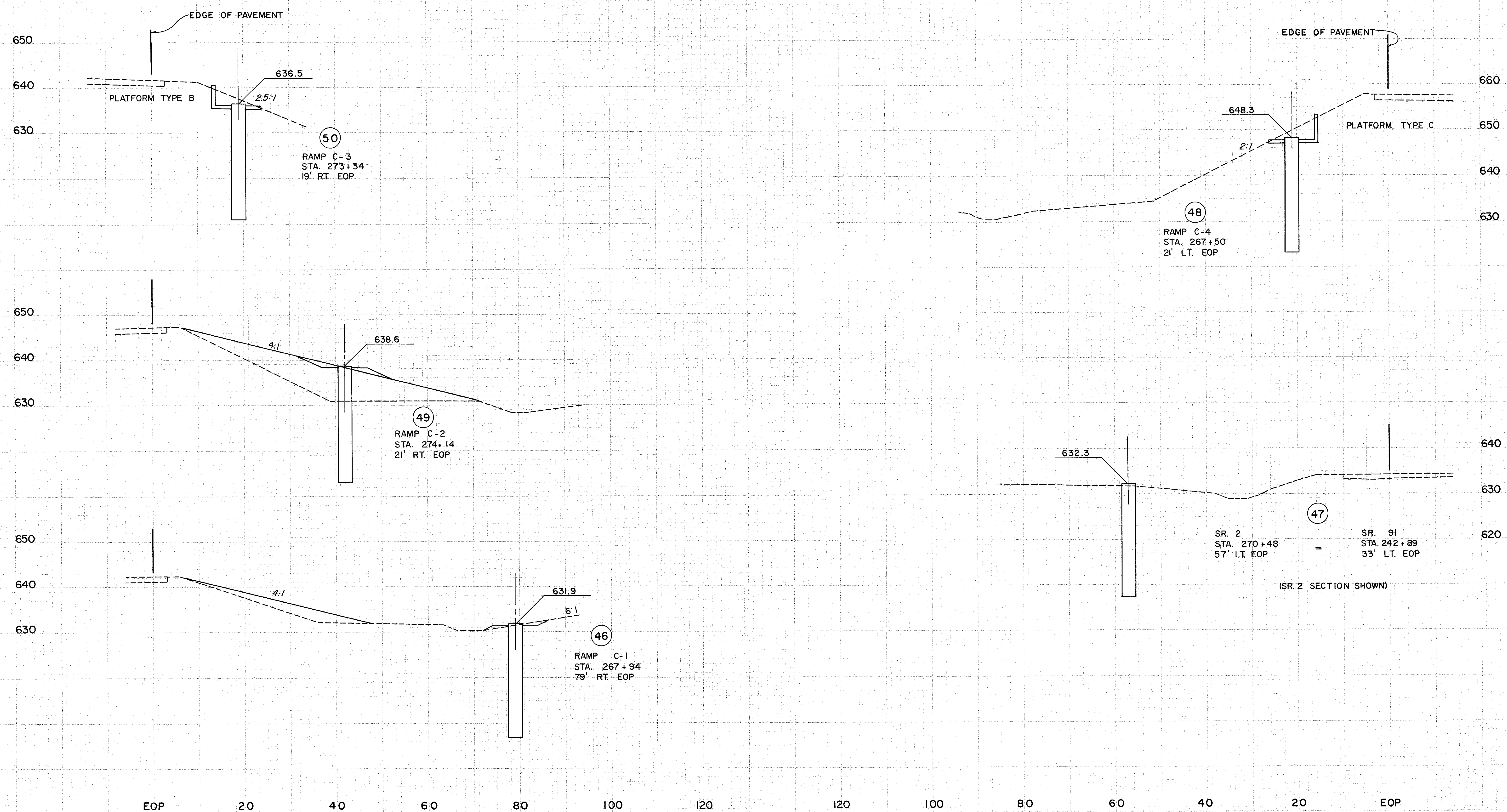
TOWER FOUNDATION CROSS SECTIONS
