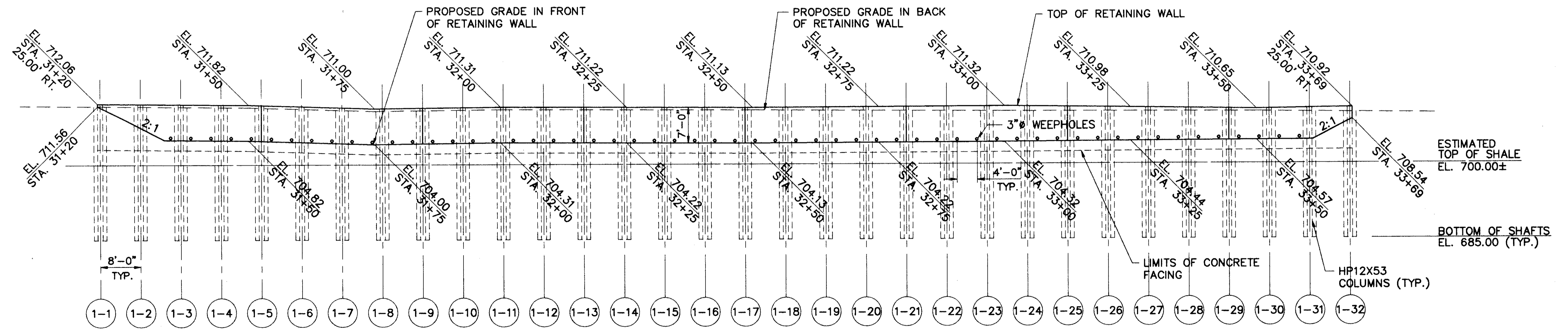
RETAINING WALL #1 ELEVATION STA. 31+20 TO STA. 33+69
