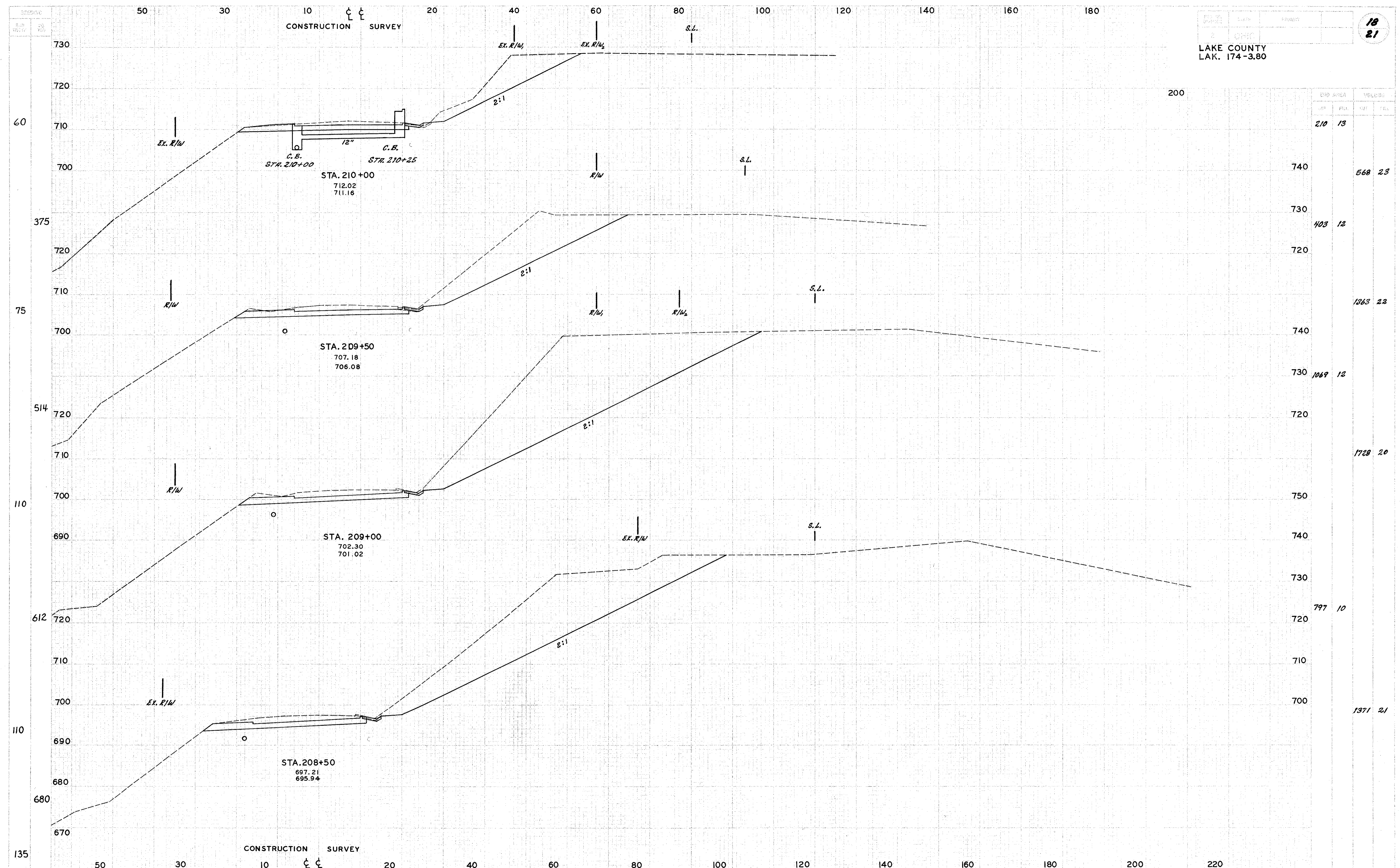
CROSS SECTIONS SR.174 STA.208+50 TO 210+00
