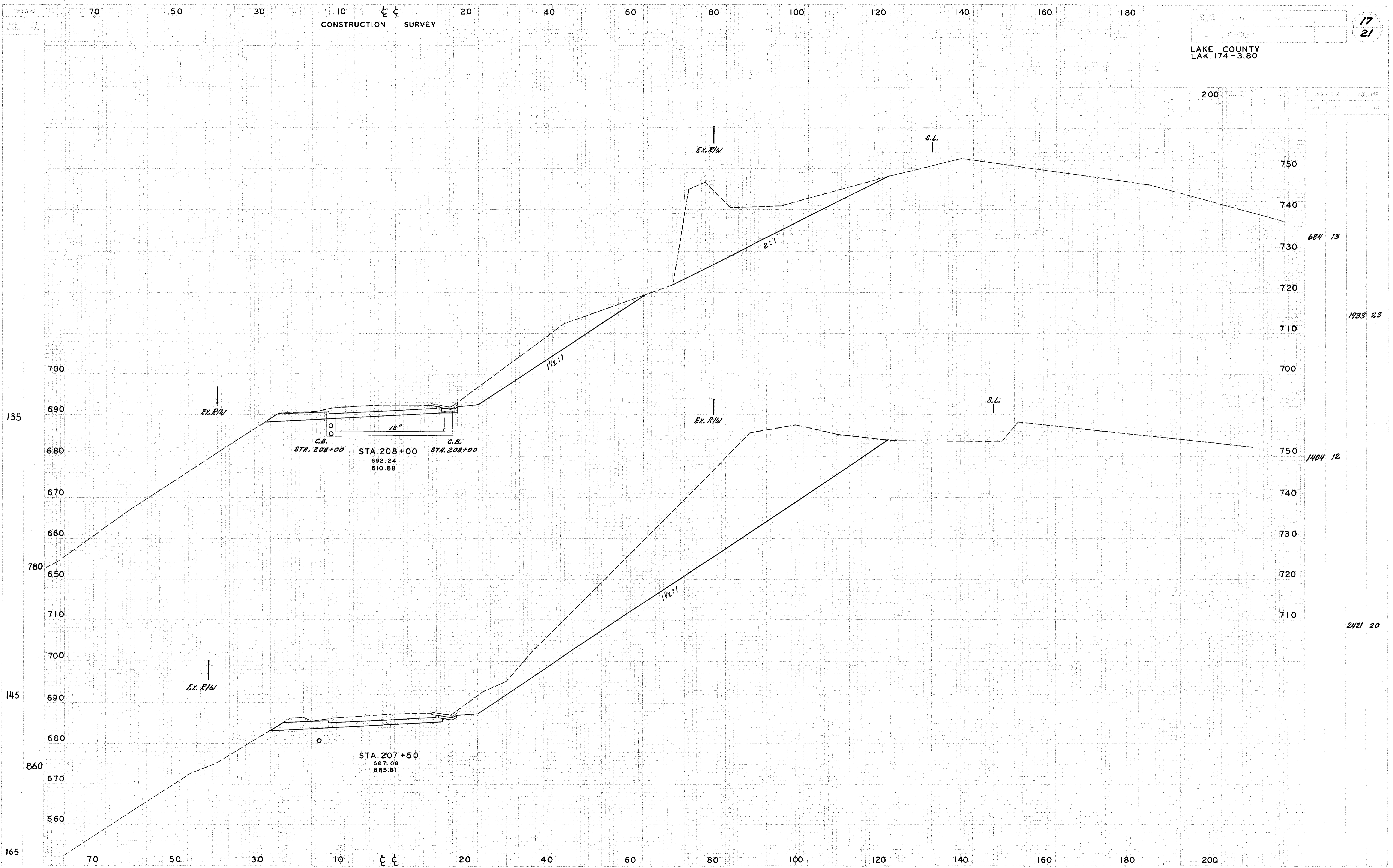
CROSS SECTIONS SR.174 STA.207+50 TO 208+00
