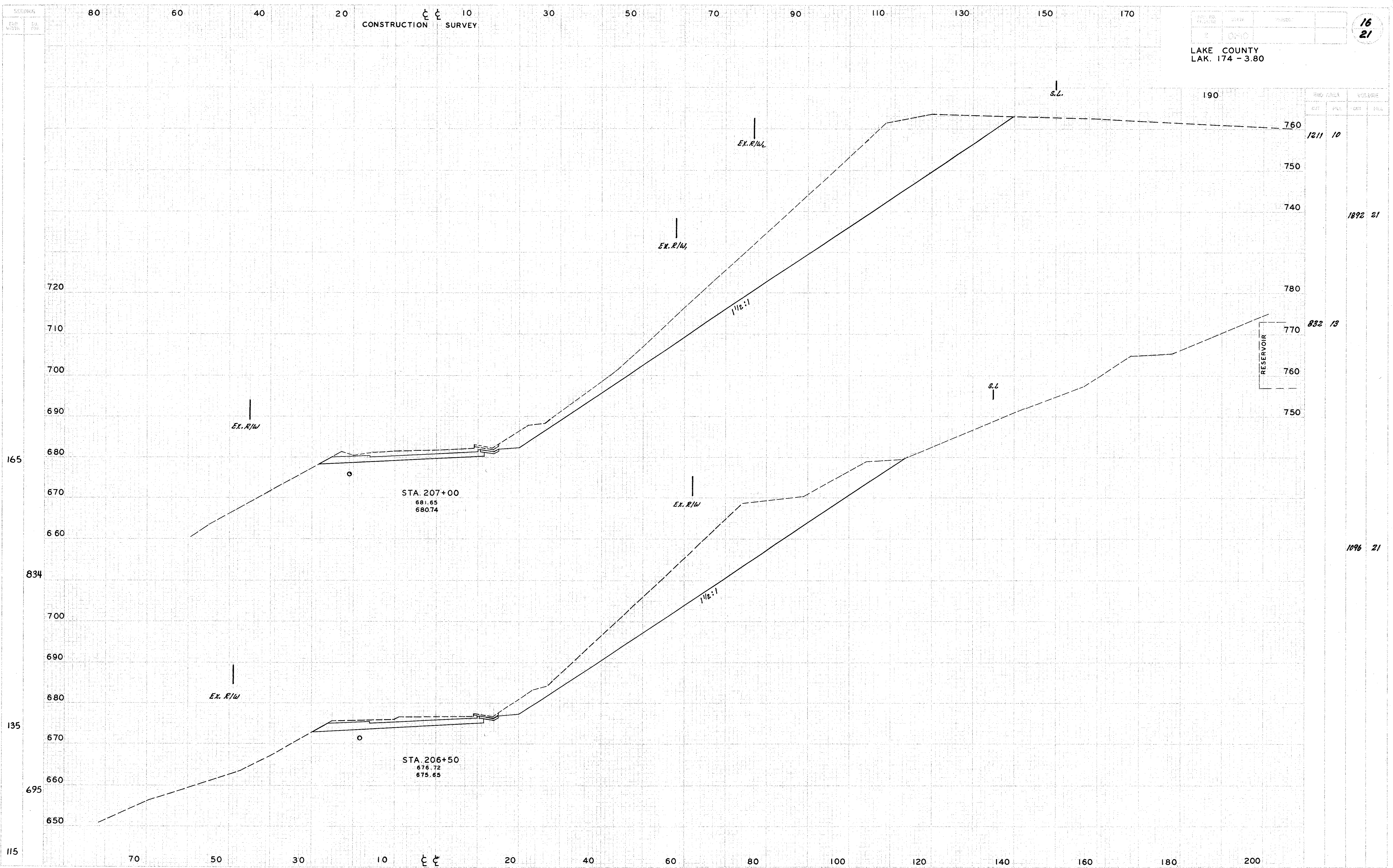
CROSS SECTIONS SR.174 STA.206+50 TO 207+00
