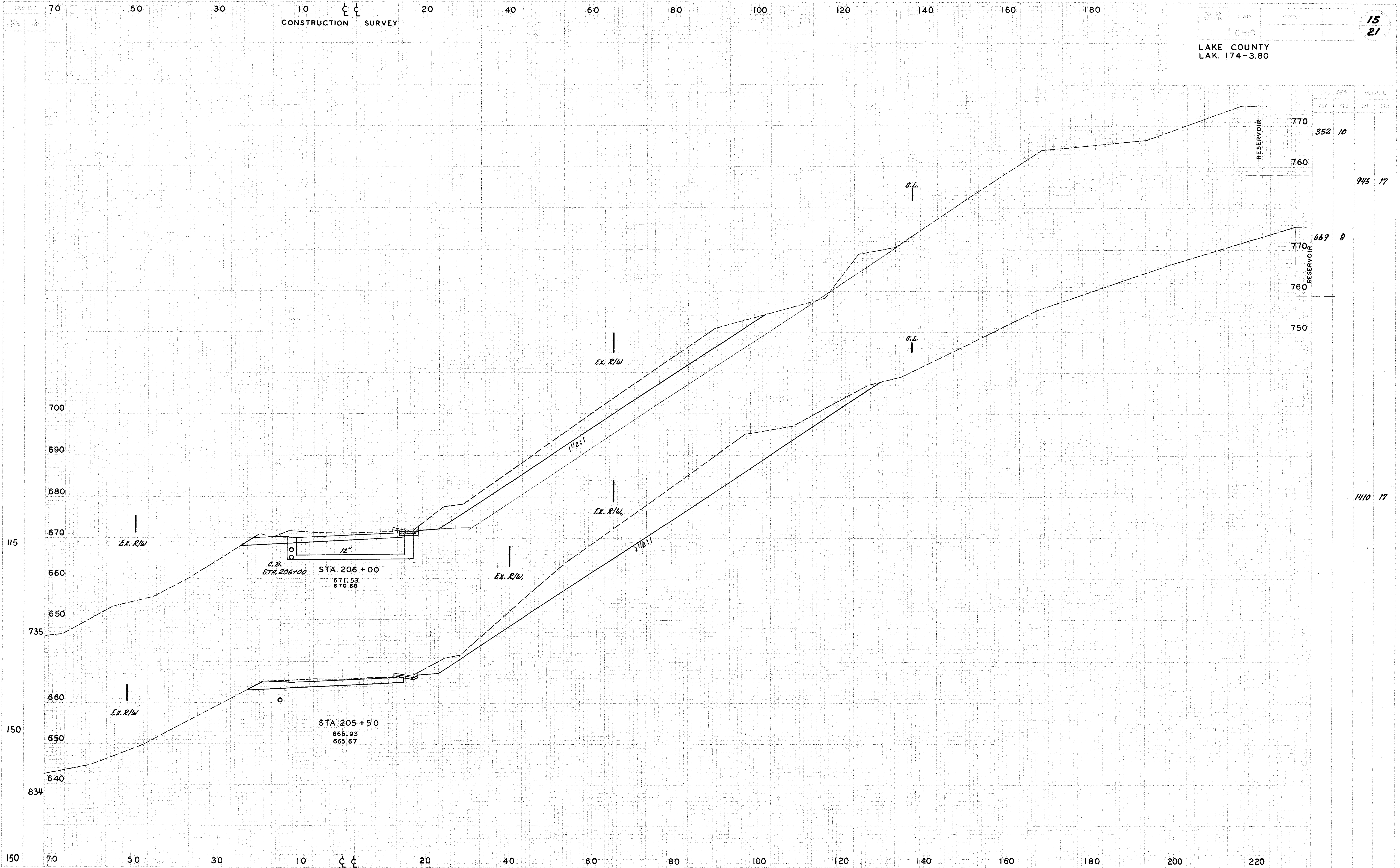
CROSS SECTIONS SR.174 STA. 205+50 TO 206+00
