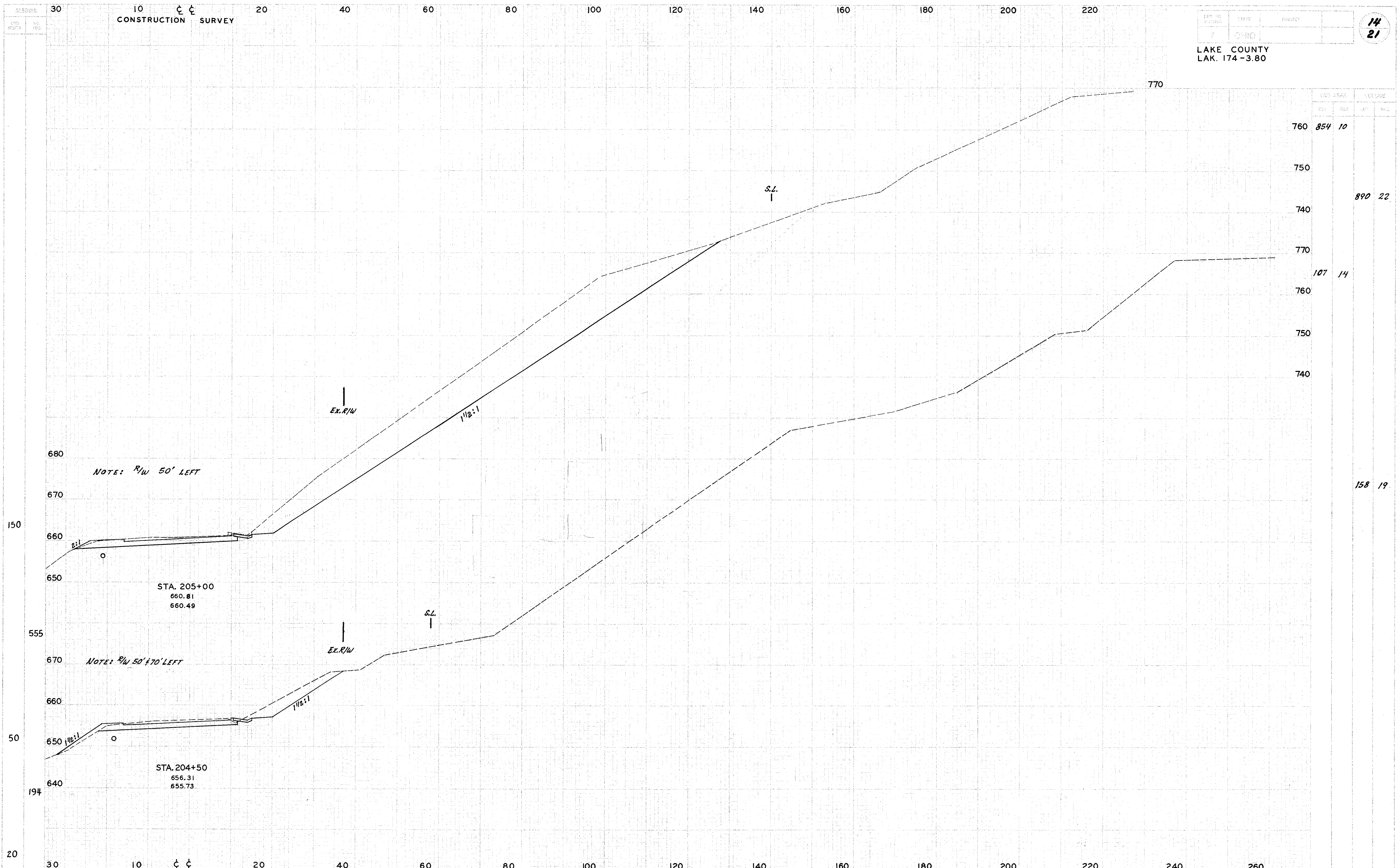
CROSS SECTIONS SR.174 STA.204+50 TO 205+00
