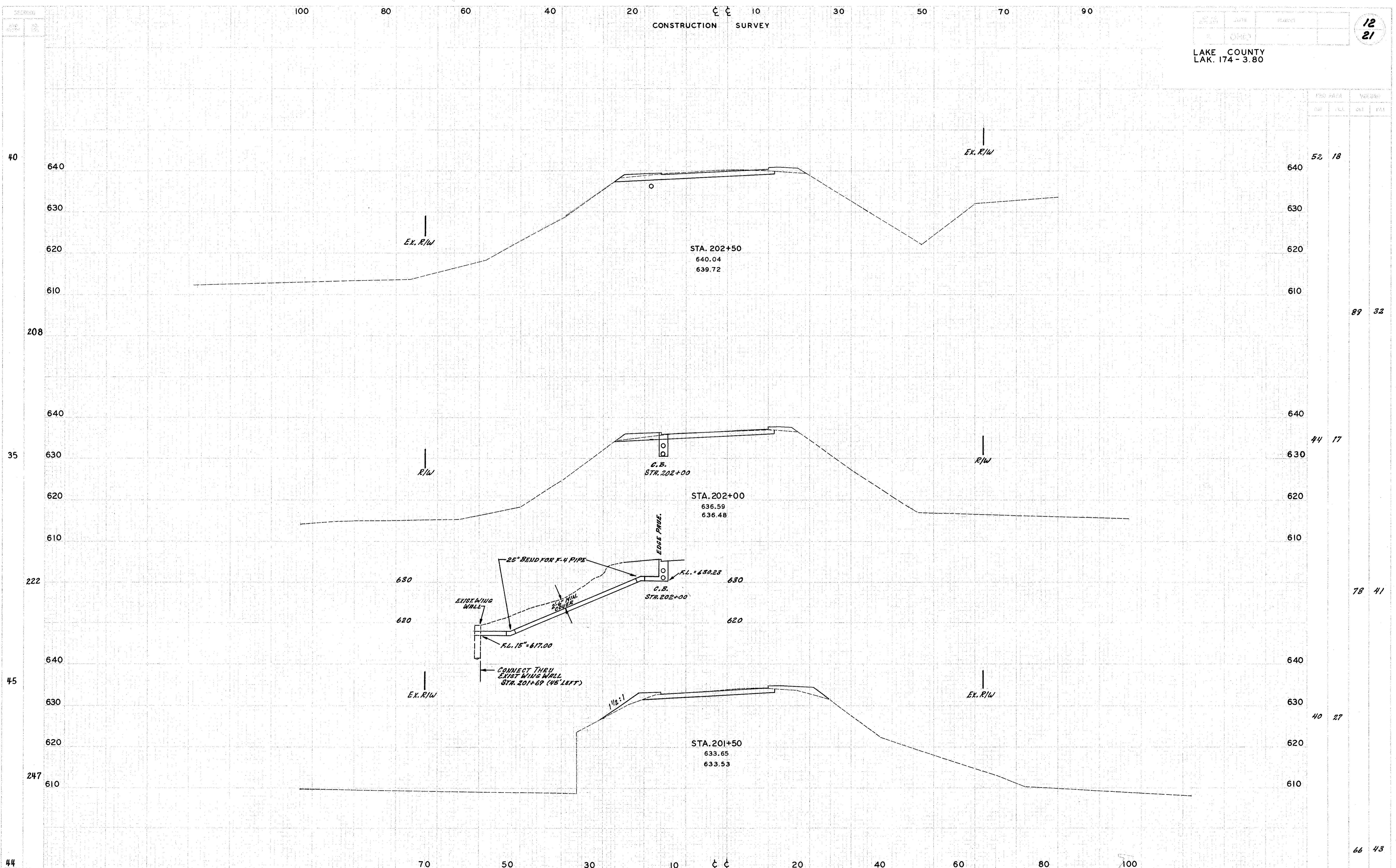
CROSS SECTIONS SR.174 STA. 201+50 TO 202+50
