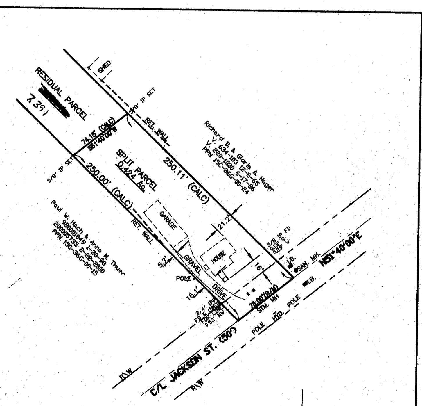
SPLIT PARCEL - ENLARGED VIEW SCALE: 1" = 60'
