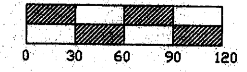
SPLIT PARCEL - ENLARGED VIEW SCALE: 1" = 60'
