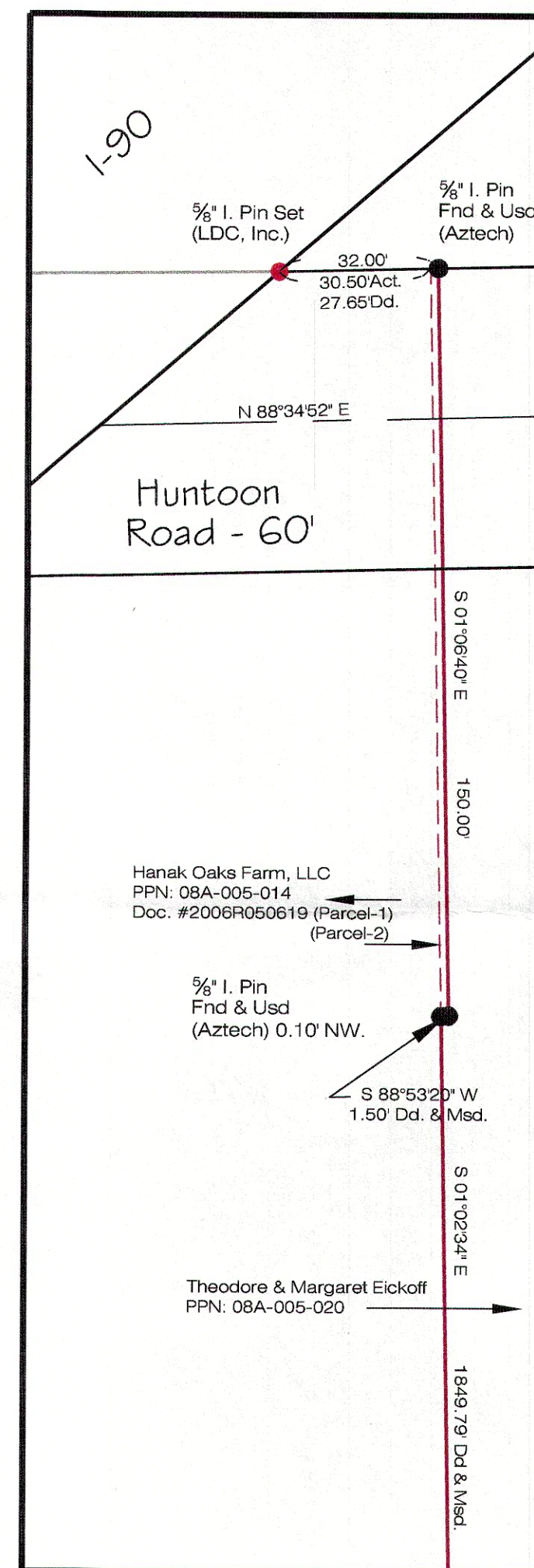
Detail: 1" = 30'
