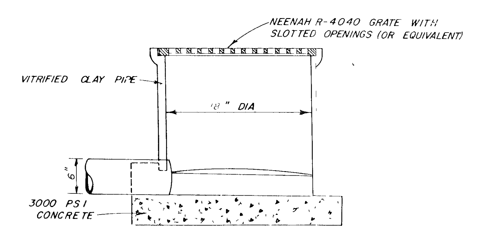
PARKING LOT INLET BASIN DETAIL
