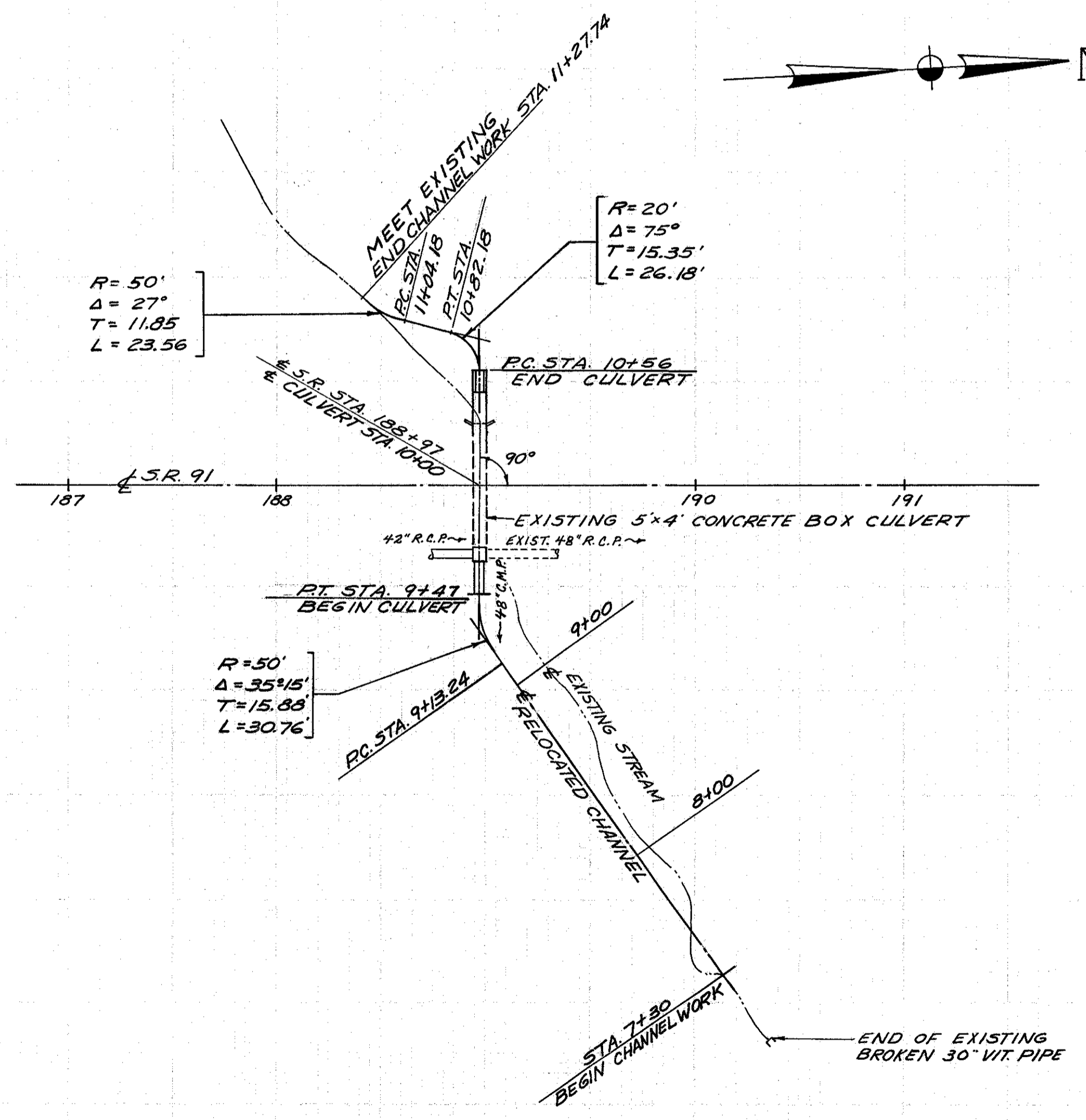
LOCATION PLAN CHANNEL RELOCATION SCALE: 1" = 50'
