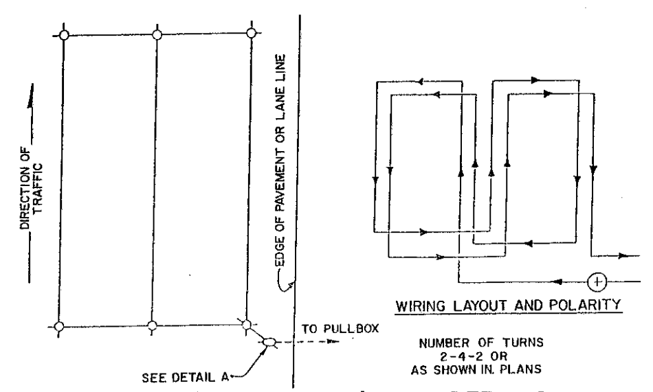
FIGURE 8 (QUADRUPOLE) LOOP DETAILS
