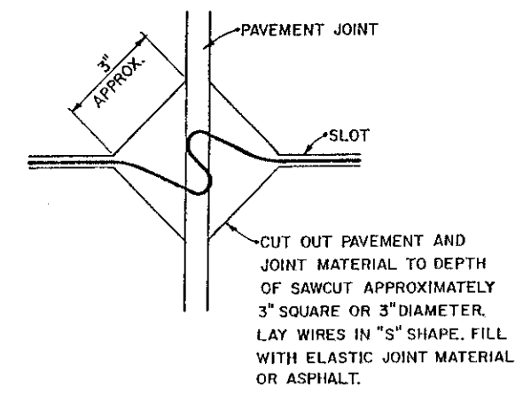
JOINT CROSSING DETAIL IN P.C.C. PAVEMENTS
