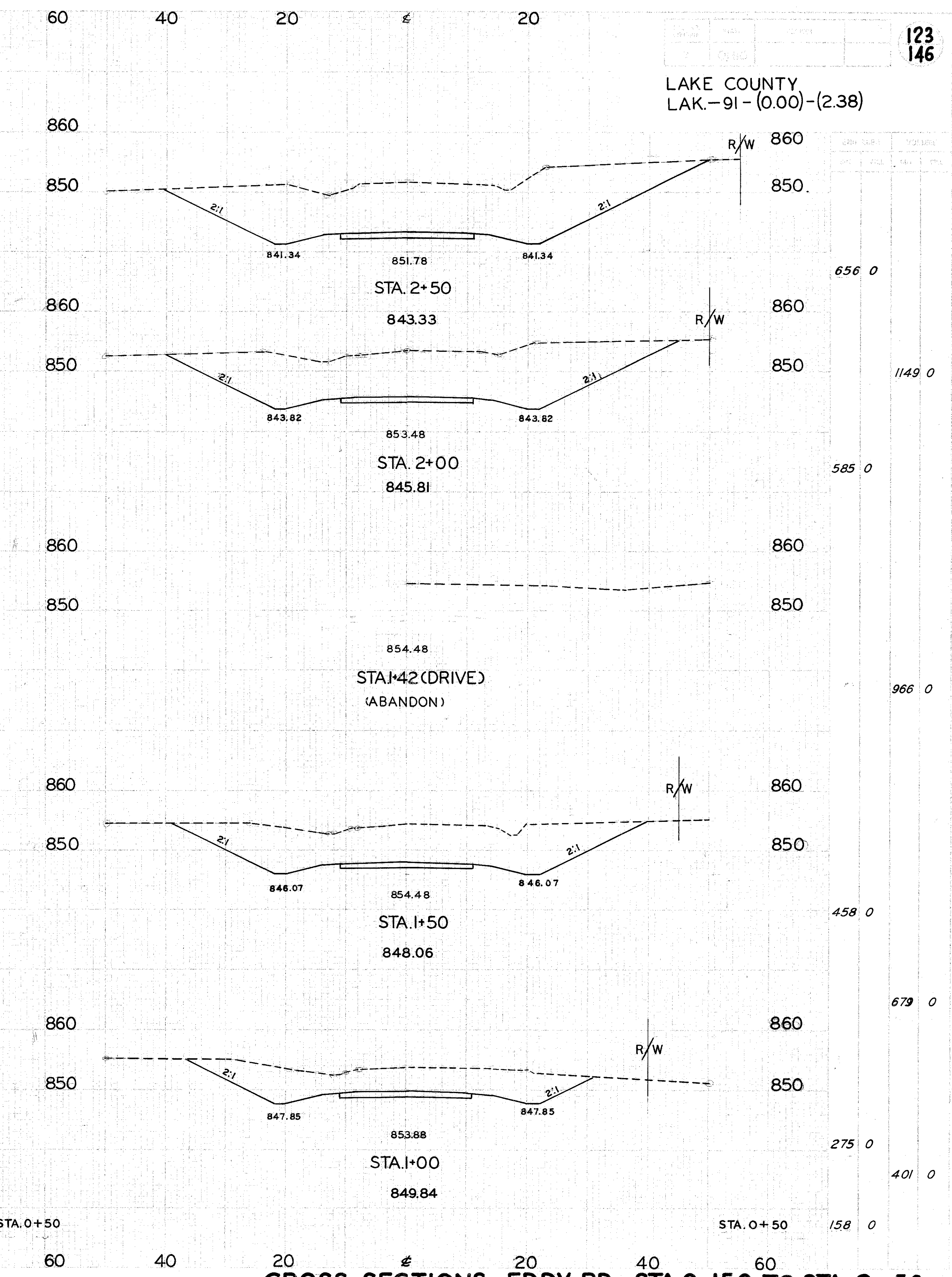
CROSS SECTIONS...EDDY RD...STA.0-150 TO STA. 2+50
