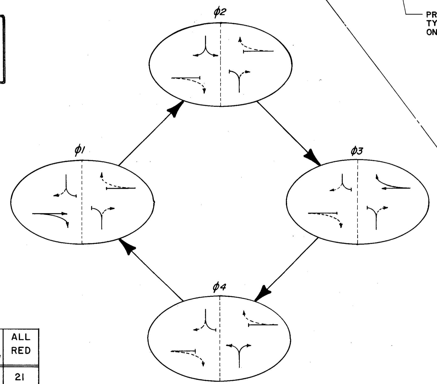
TEMPORARY PHASING DIAGRAM (FOR BOTH PHASES OF CONSTRUCTION)
