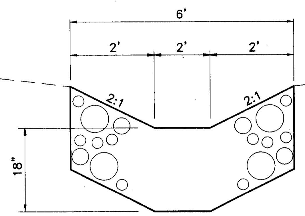
ITEM 601 - ROCK CHANNEL PROTECTION TYPE C, WITH FILTER AS PER STD. DWG. HW-2.2
