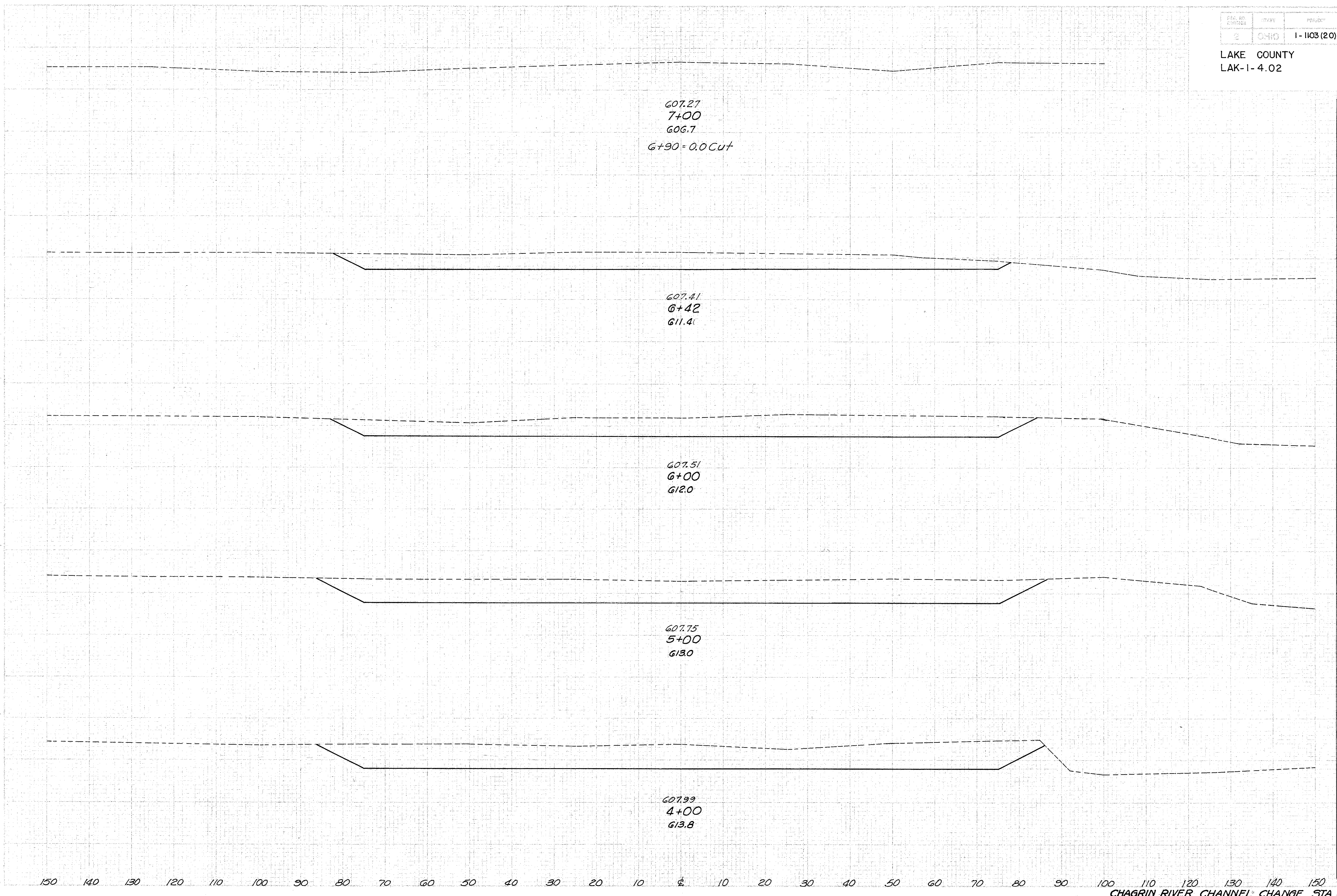
CHAGRIN RIVER CHANNEL CHANGE STA. 4+00 to 7+00
