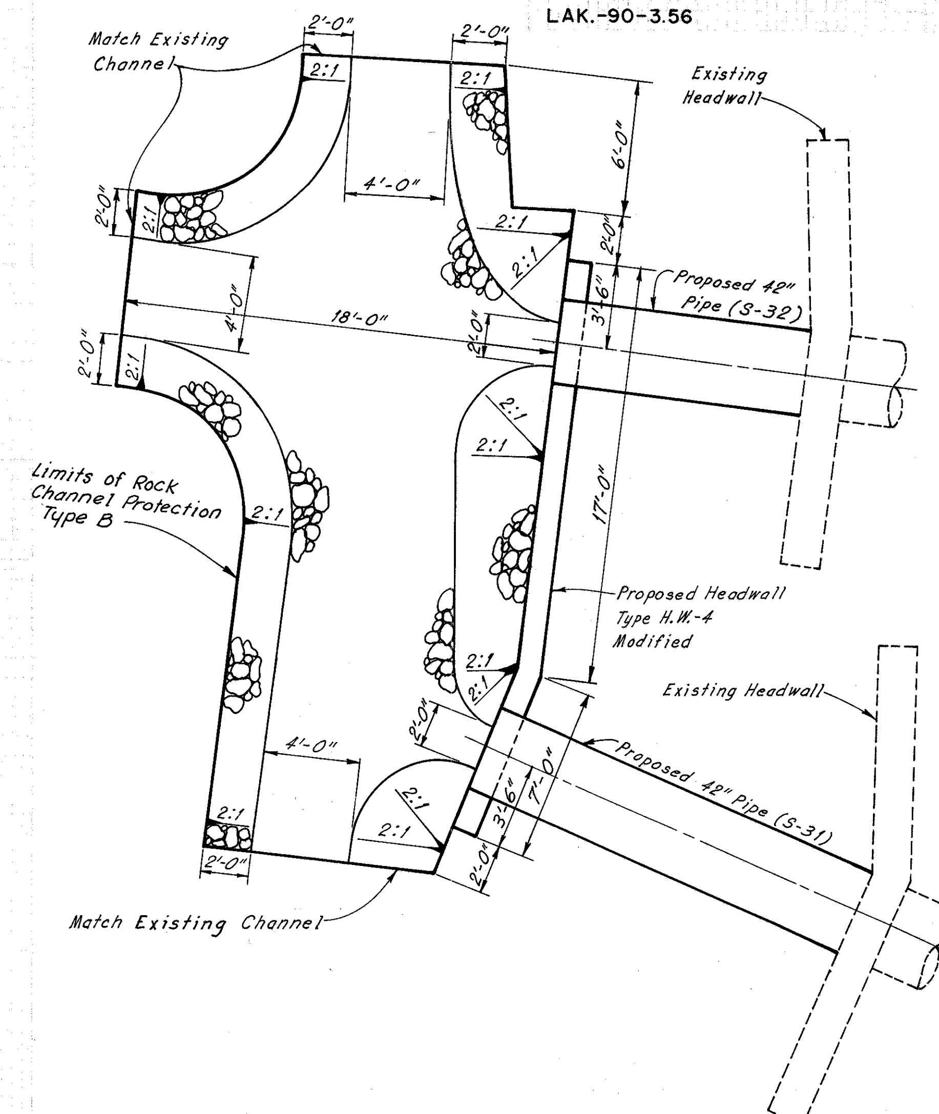
PLAN ROCK CHANNEL PROTECTION, TYPE B, S-31 & S-32 Scale: 1/4" = 1'-0"
