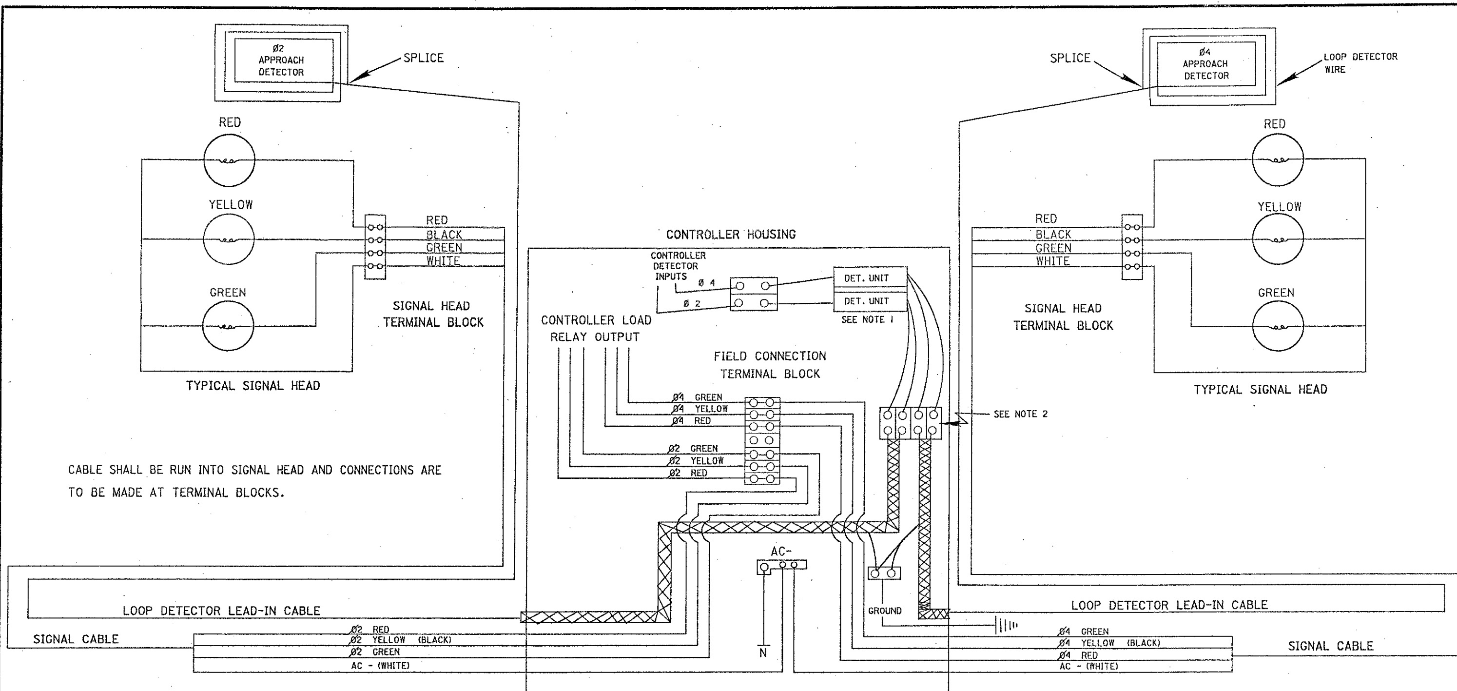
TYPICAL SIGNAL HEAD HOOK-UP
