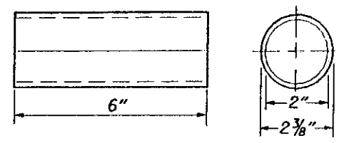
POST SLEEVE
