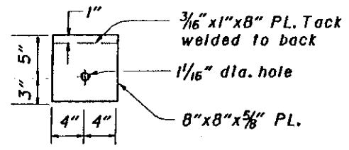
BEARING PLATE
