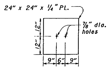
SOIL PLATE
