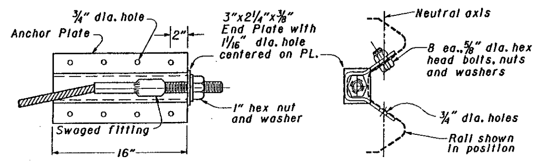
ANCHOR PLATE ASSEMBLY DETAILS
