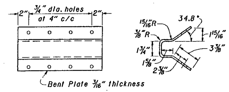
ANCHOR PLATE
