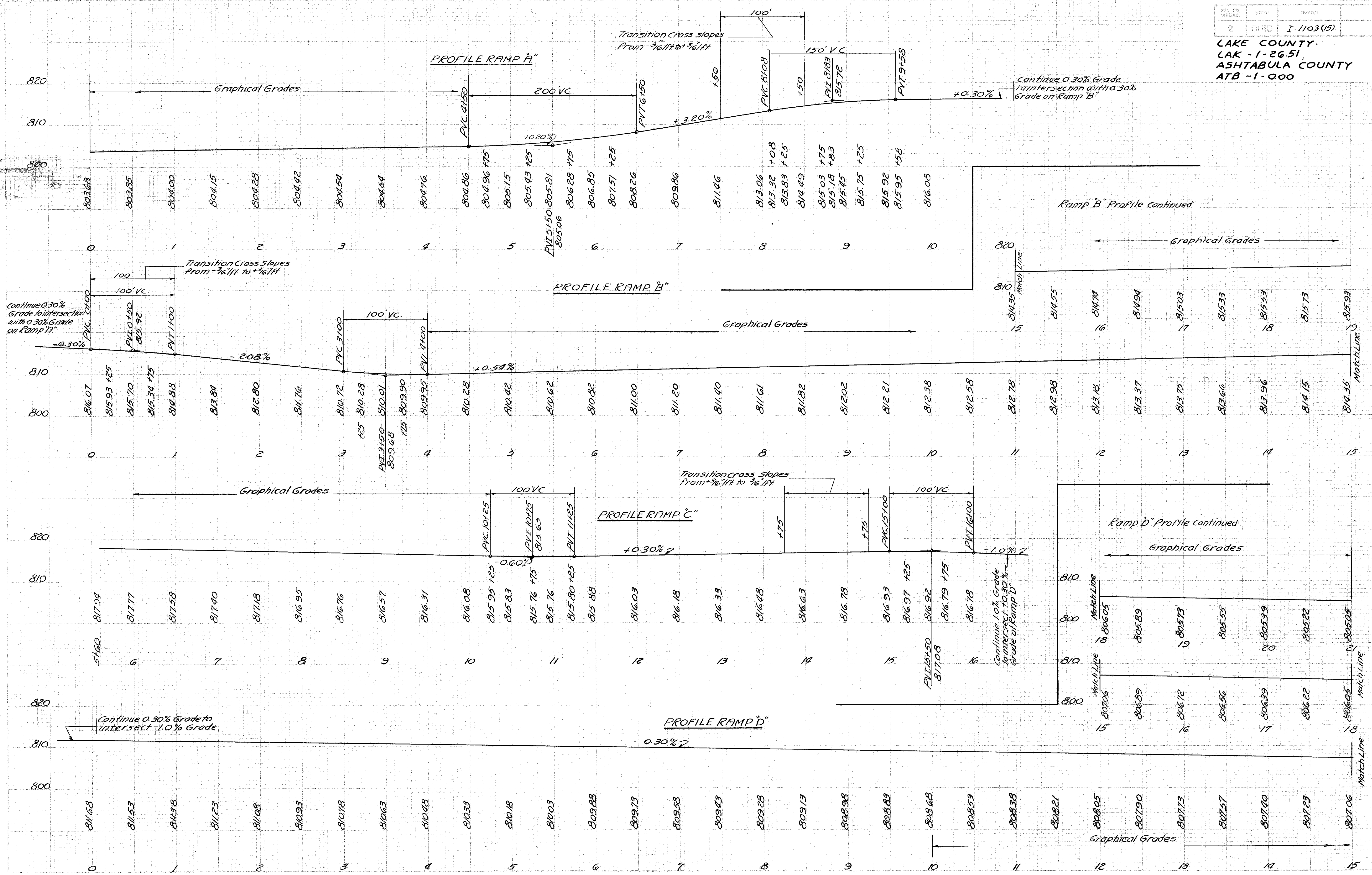
ROADSIDE REST RAMP GRADES
