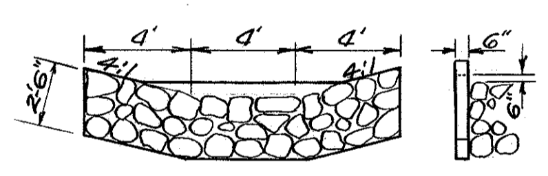
Section A-A Dumped Rock Channel Protection With Conc. Endsill
