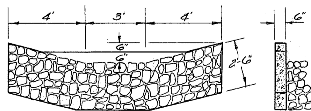
SECTION A-A DUMPED ROCK CHANNEL PROTECTION WITH CONCRETE ENDSILL
