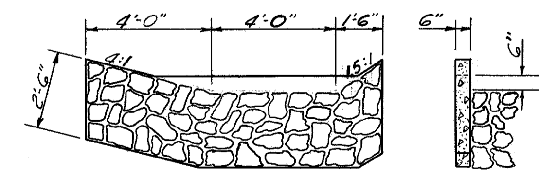
Section A-A Dumped Rock Channel Protection With Concrete Endsill
