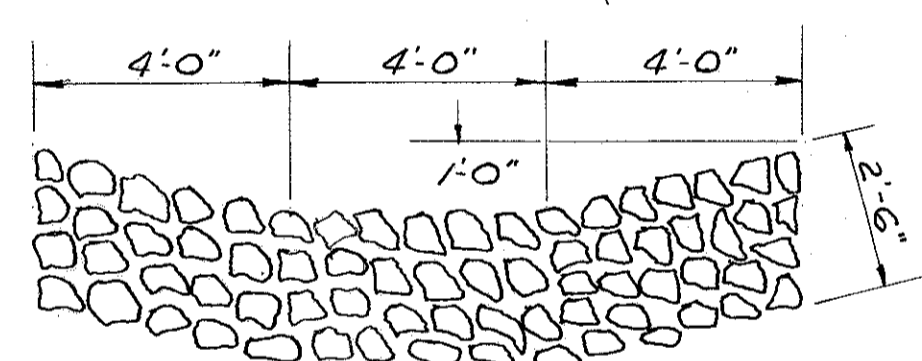
Section A-A DUMPED ROCK CHANNEL PROTECTION
