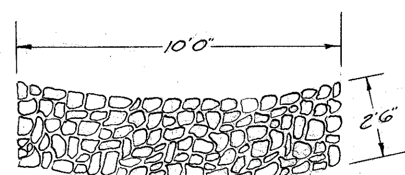
SECTION A-A DUMPED ROCK CHANNEL PROTECTION
