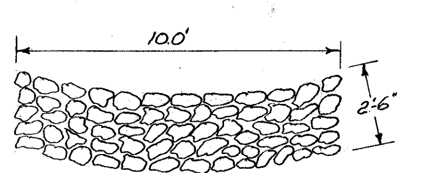
SECTION A-A Dumped Rock Channel Protection
