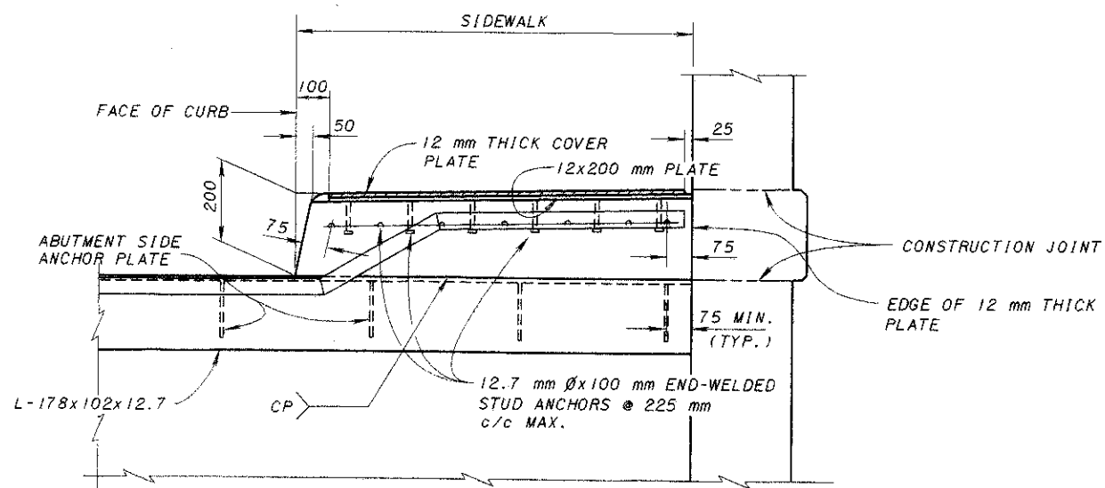
SECTION F-F
