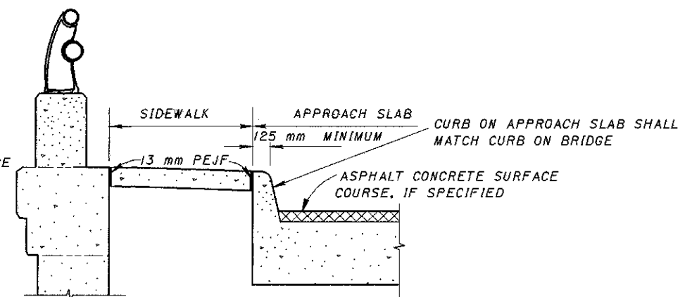
SECTION C-C
