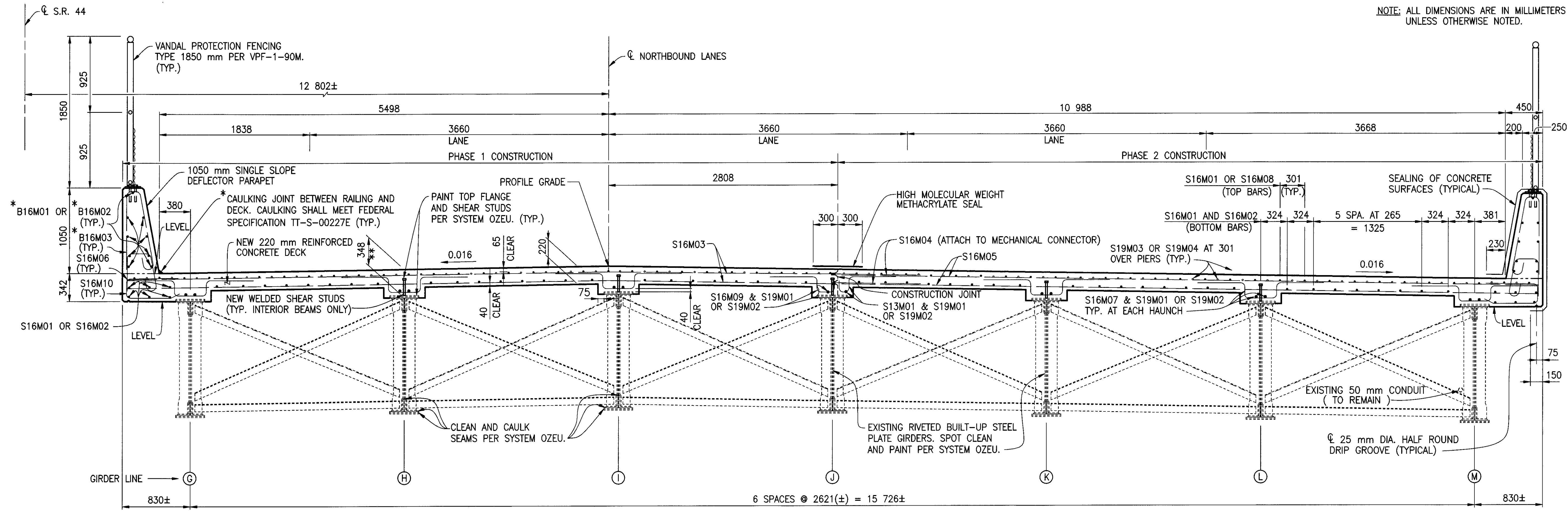
PROPOSED TRANSVERSE SECTION (NORTHBOUND BRIDGE LAK-90-23.641)
