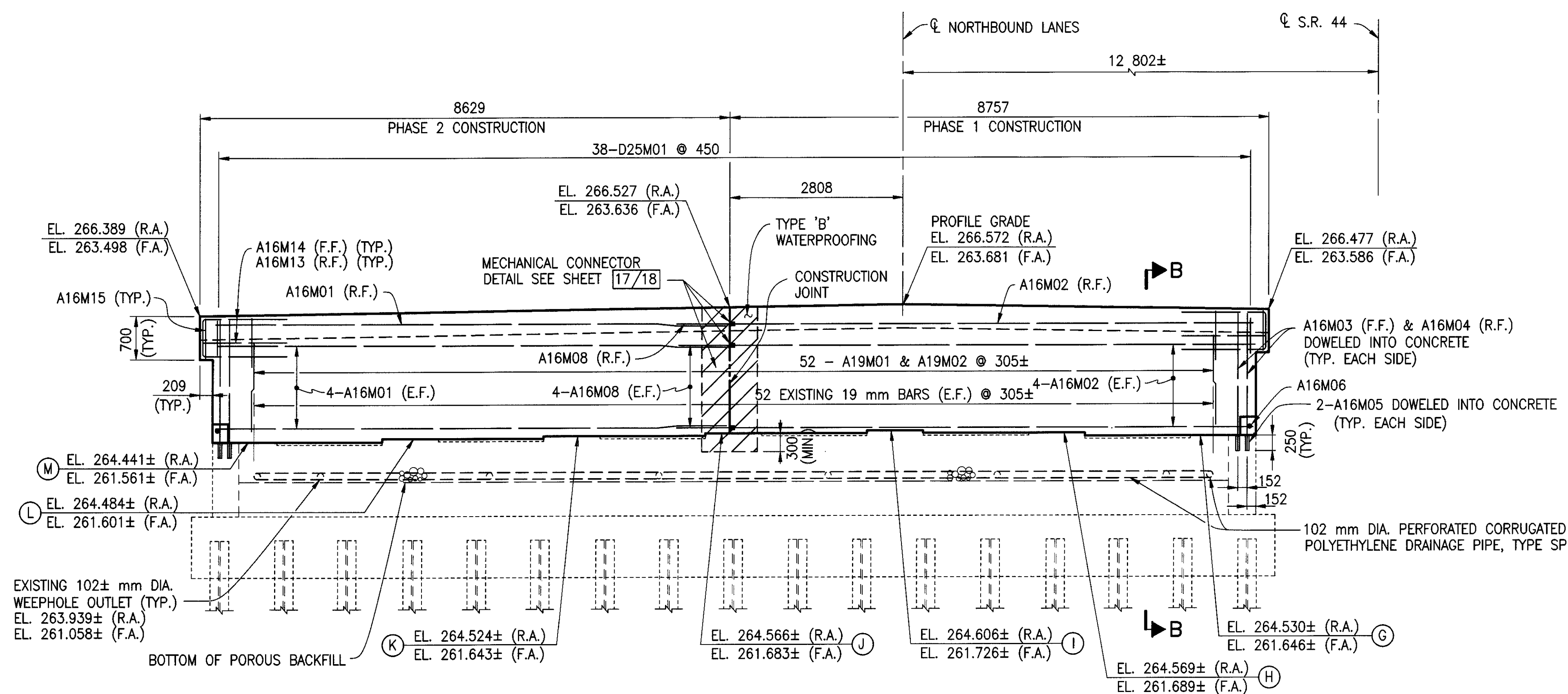
REAR ABUTMENT ELEVATION (NORTHBOUND BRIDGE LAK-90-23641) (FORWARD ABUTMENT OPPOSITE HAND)
