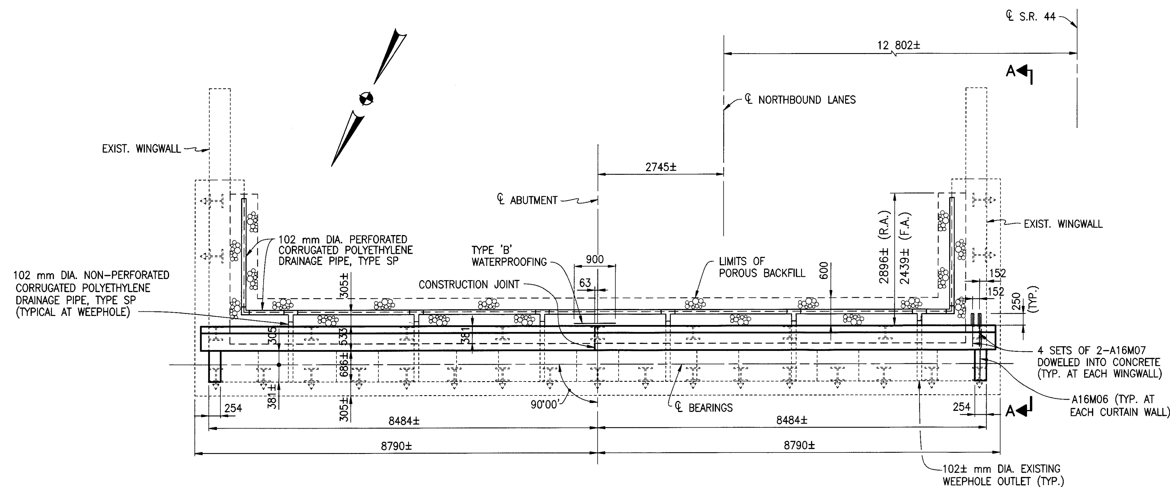
REAR ABUTMENT PLAN (NORTHBOUND BRIDGE LAK-90-23641) (FORWARD ABUTMENT OPPOSITE HAND)
