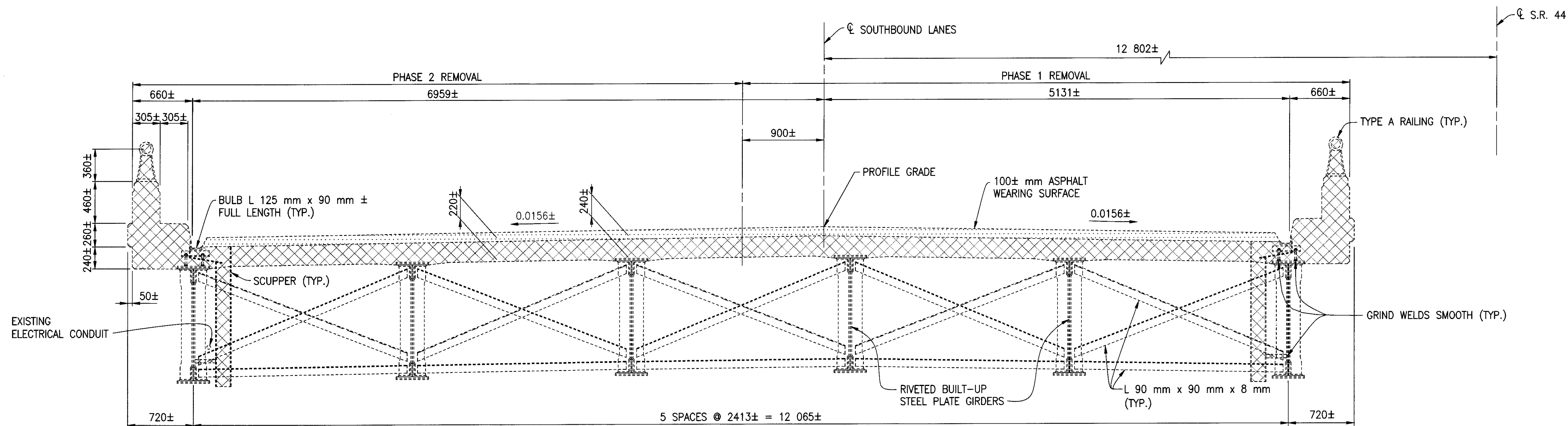
EXISTING TRANSVERSE SECTION (SOUTHBOUND BRIDGE LAK-90-23609)
