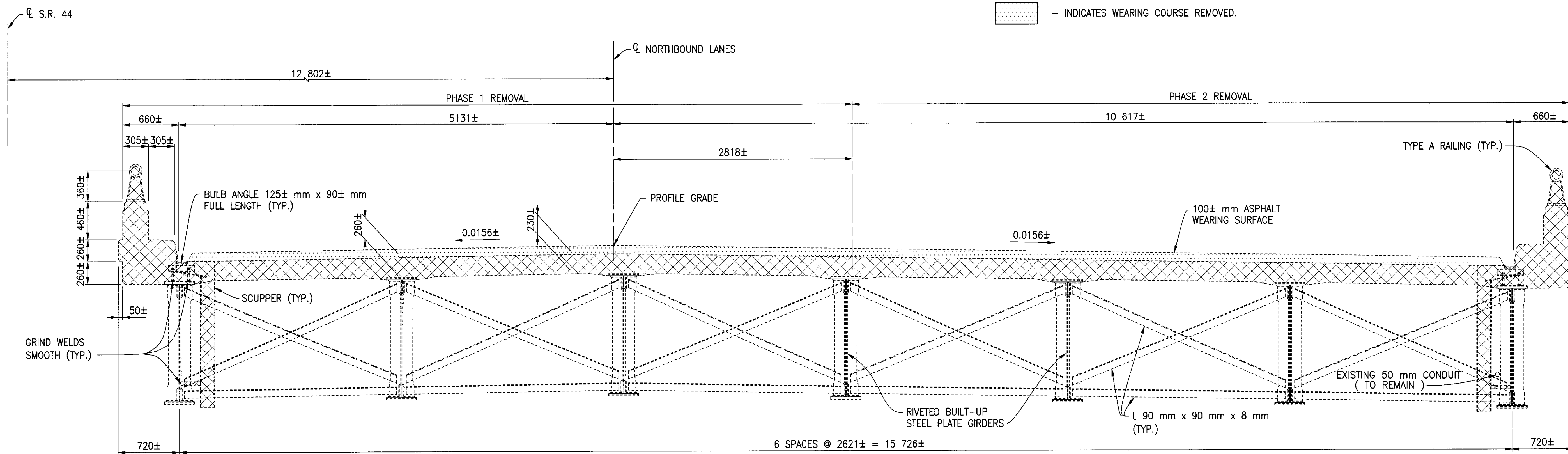
EXISTING TRANSVERSE SECTION (NORTHBOUND BRIDGE LAK-90-23641)
