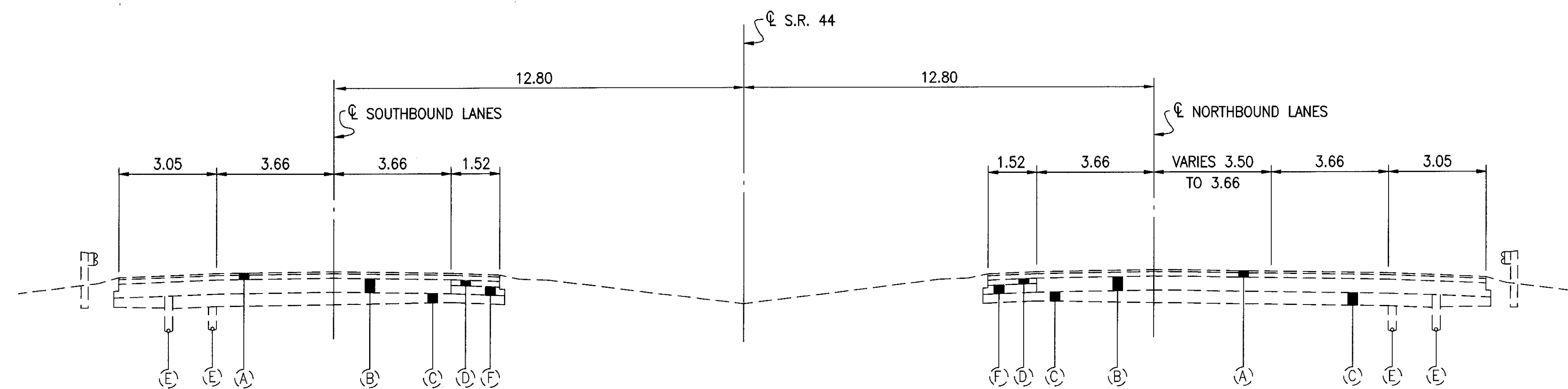
EXISTING TYPICAL SECTION
