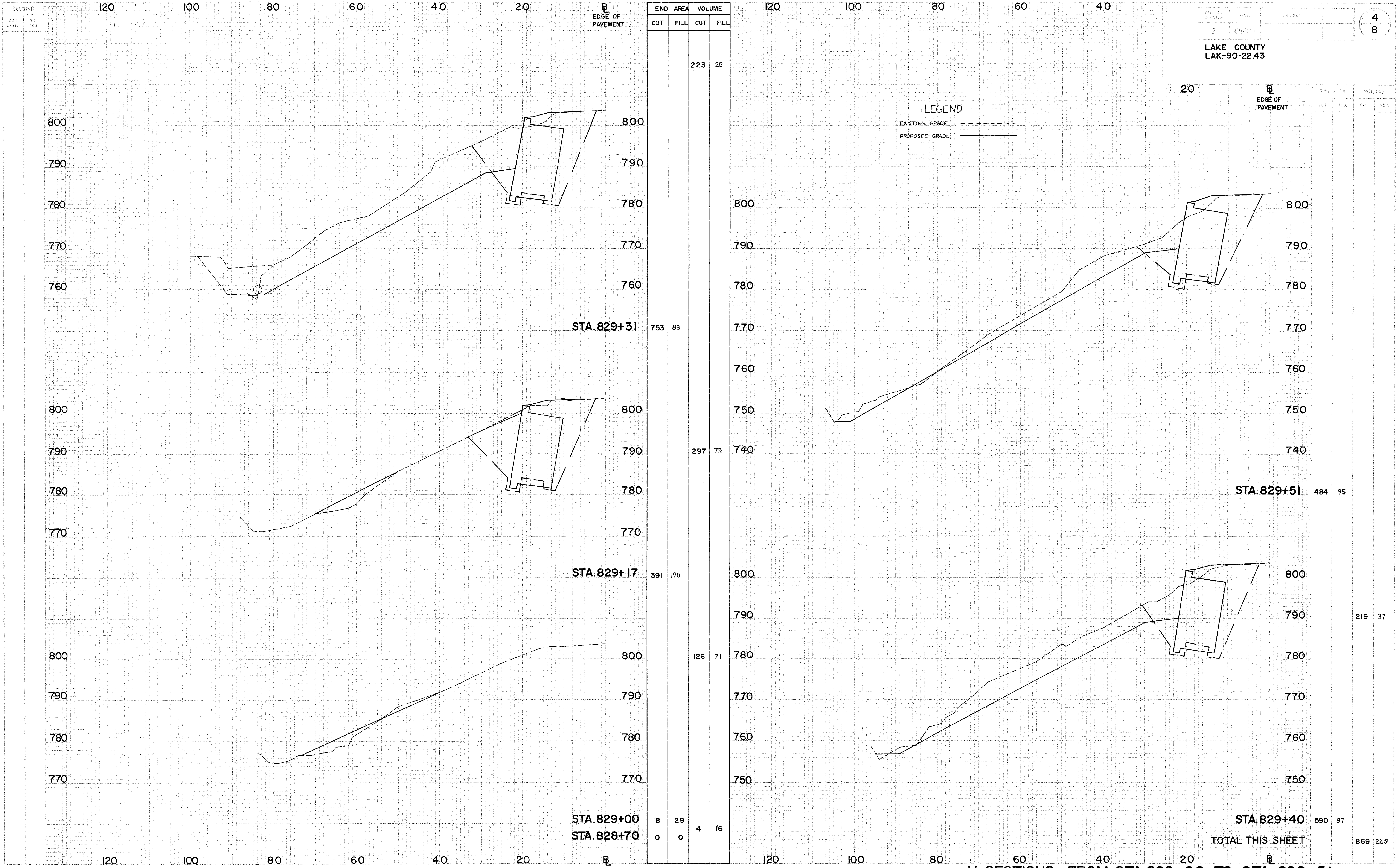
X-SECTIONS - FROM STA. 829+00 TO STA. 829+51
