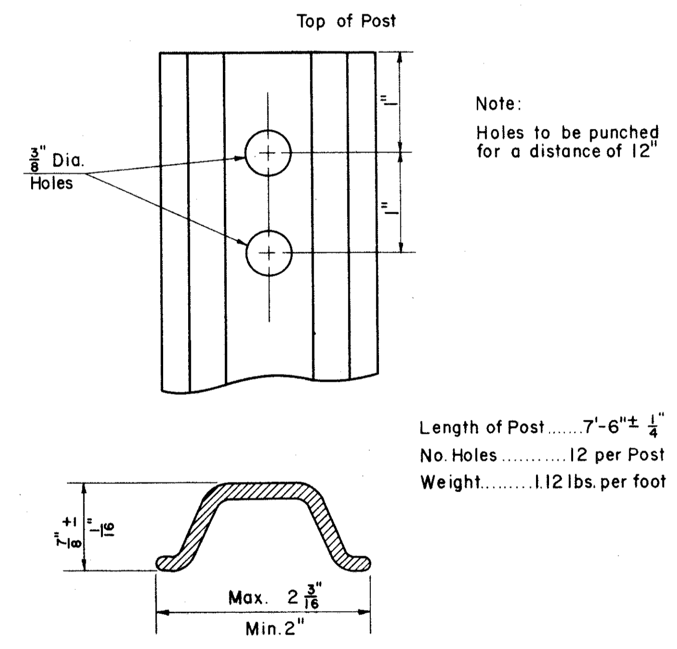
SECTION VIEW DETAIL OF STEEL DRIVE POST FOR DELINEATOR
