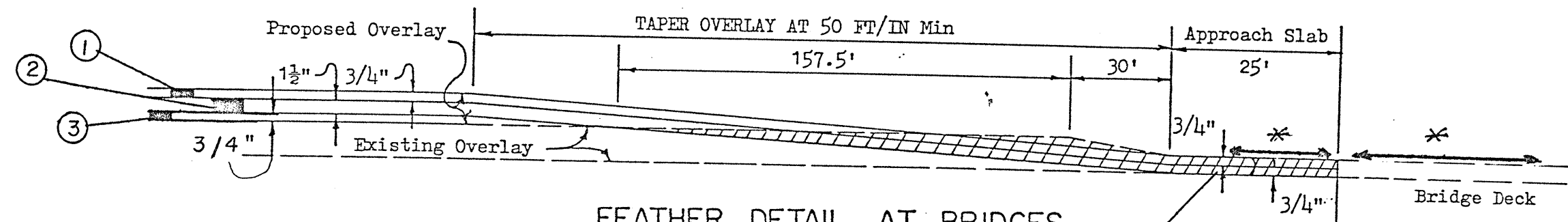
FEATHER DETAIL AT BRIDGES (NO SCALE)
