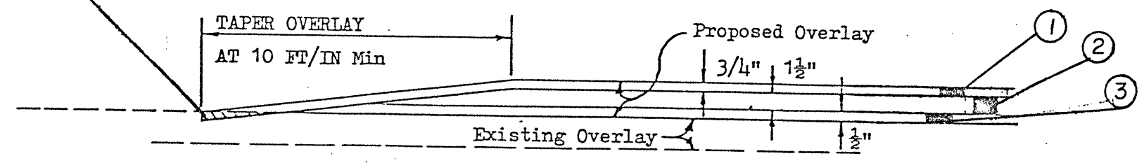
FEATHER DETAIL AT RAMPS (NO SCALE)
