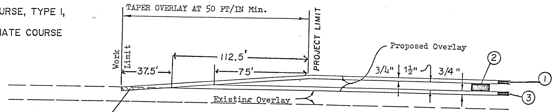
FEATHER DETAIL (NO SCALE)
