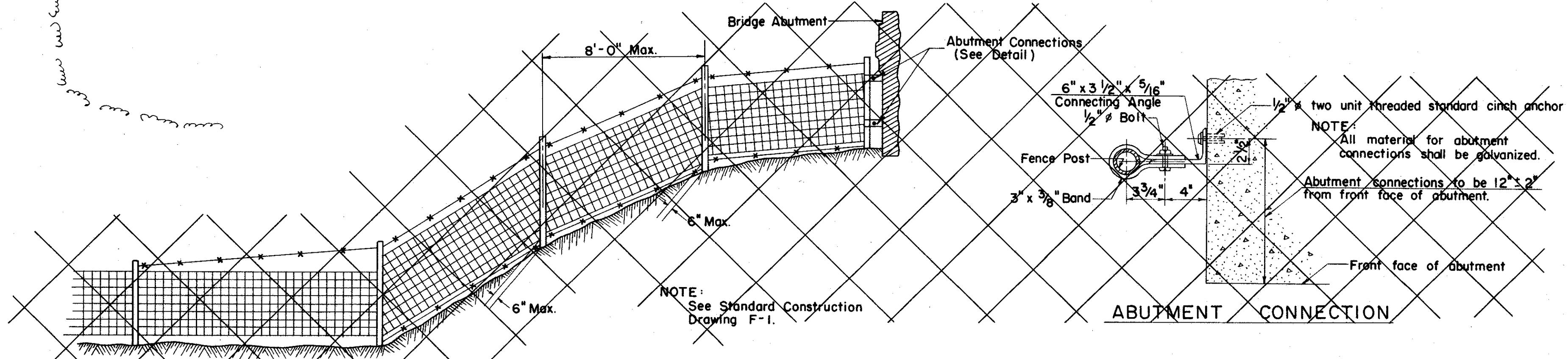
TYPE "A" FENCE SCALE: 1/4" = 1'-0"
