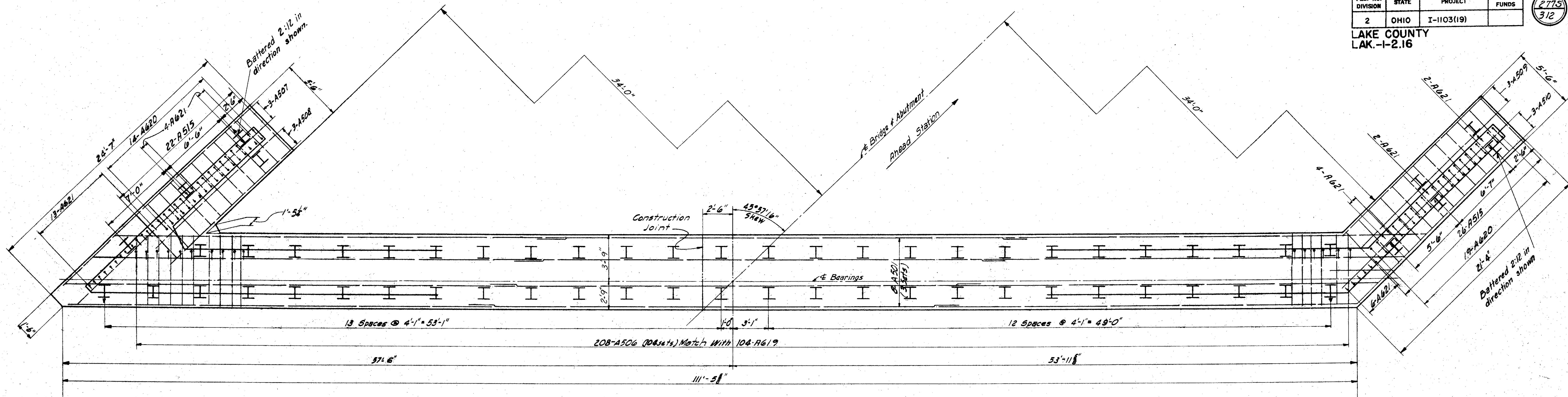
FOOTING PLAN ABUTMENT NO. 2
