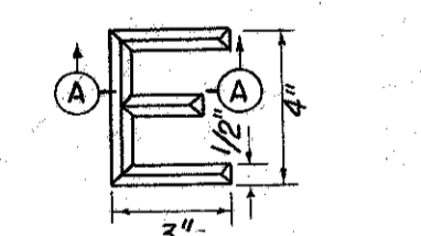
TYPICAL SYMBOL Scale: 3/16"=1' Dimensions shown are for all symbols impressed in Concrete Marker
